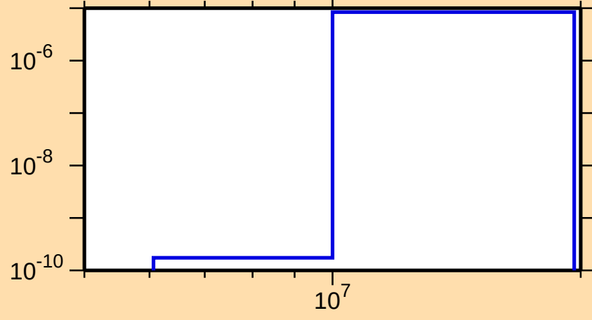
\sigma vs. E for ^{224}\text{Po}(n,\alpha)
