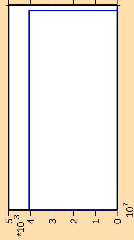
\Delta\sigma/\sigma vs. E for ^{224}\text{Po}(\text{mt } 11)
