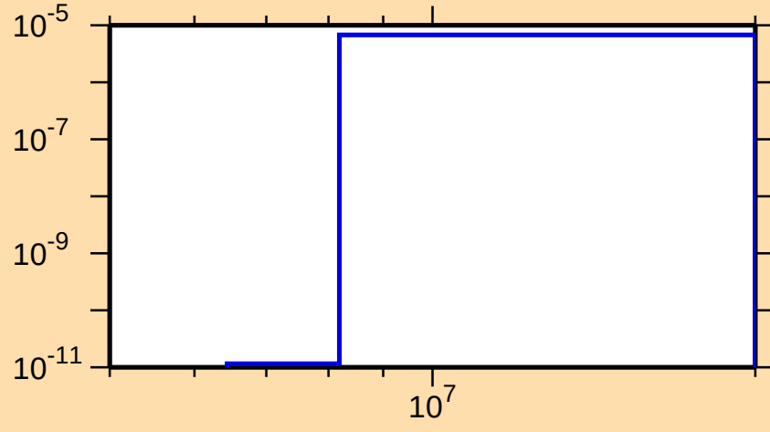
\sigma vs. E for ^{224}\text{Po}(n,\alpha)
