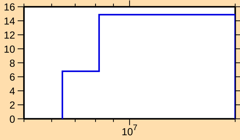
\Delta\sigma/\sigma vs. E for ^{224}\text{Po}(n,\text{nonel.})
