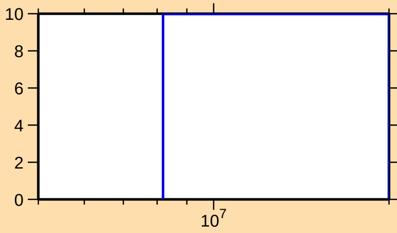
\Delta\sigma/\sigma vs. E for ^{224}\text{Po}(n,\text{inel.})
