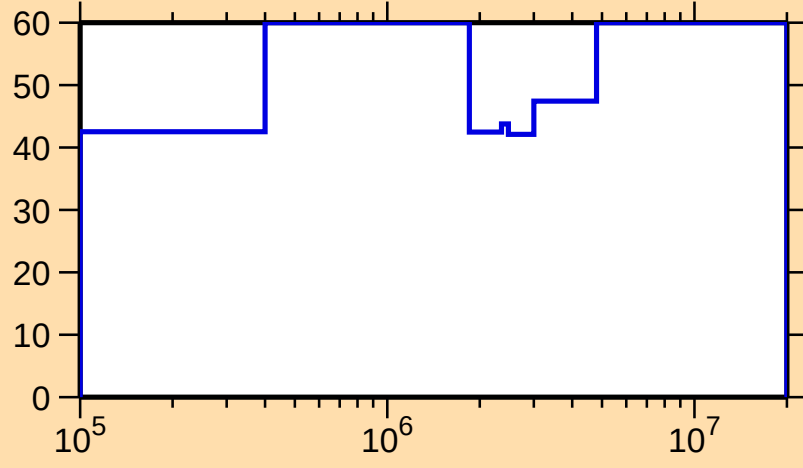
\Delta\sigma/\sigma vs. E for ^{224}\text{Po}(n,\text{el.})
