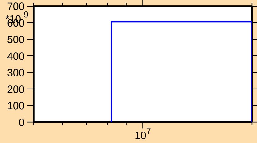
\sigma vs. E for ^{224}\text{Po}(n,np)
