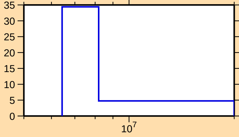
\Delta\sigma/\sigma vs. E for ^{224}\text{Po}(n,\text{ncont.})
