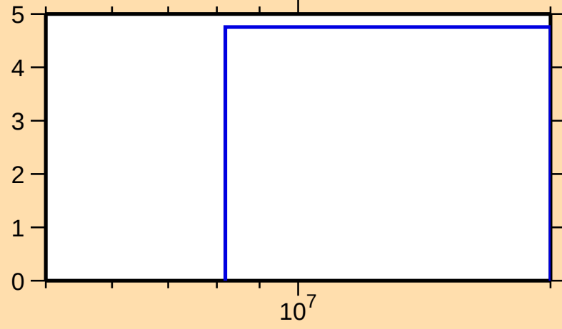
\Delta\sigma/\sigma vs. E for ^{224}\text{Po}(n,n\text{cont.})
