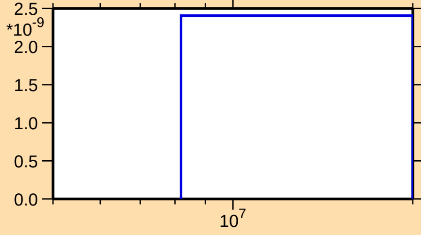
\sigma vs. E for ^{224}\text{Po}(n,2n\alpha)
