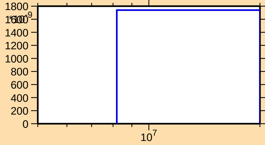
\sigma vs. E for ^{224}\text{Po}(n,d)
