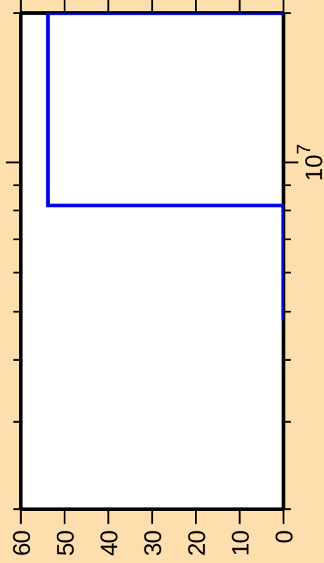
\Delta\sigma/\sigma vs. E for ^{224}\text{Po}(n,f)
