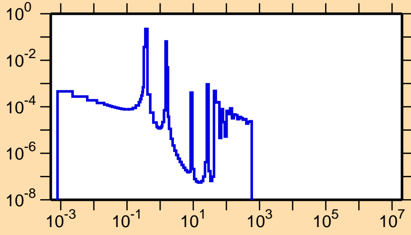
\sigma vs. E for ^{225}\text{Po}(n,f)
