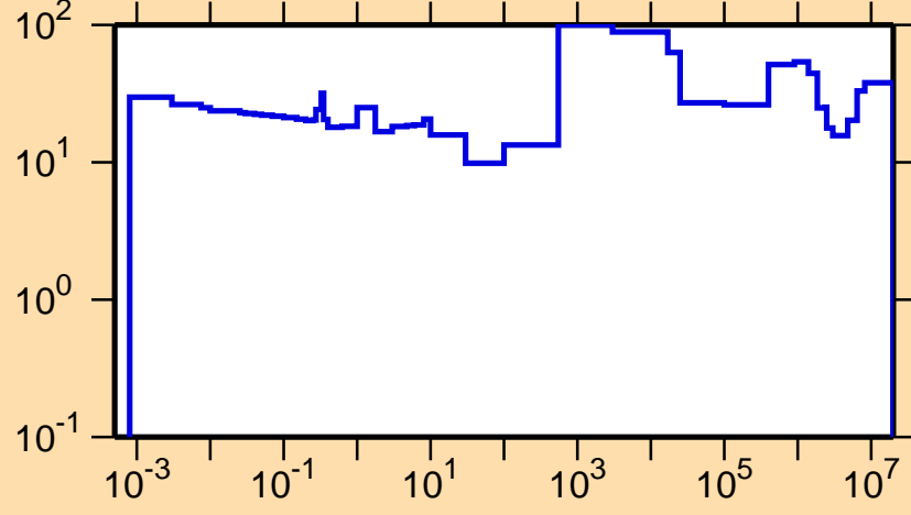
\Delta\sigma/\sigma vs. E for ^{225}\text{Po}(n,tot.)
