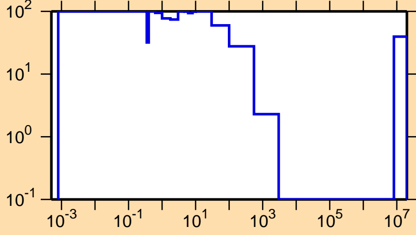
\Delta\sigma/\sigma vs. E for ^{225}\text{Po}(n,f)
