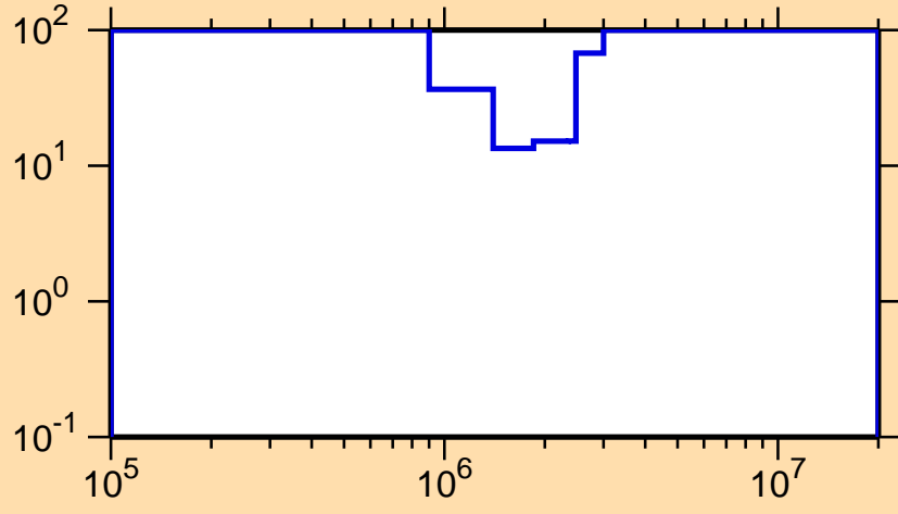
\Delta\sigma/\sigma vs. E for ^{225}\text{Po}(n,\text{inel.})
