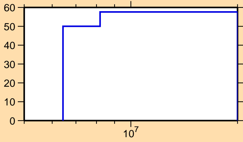
\Delta\sigma/\sigma vs. E for ^{225}\text{Po}(n,\text{el.})
