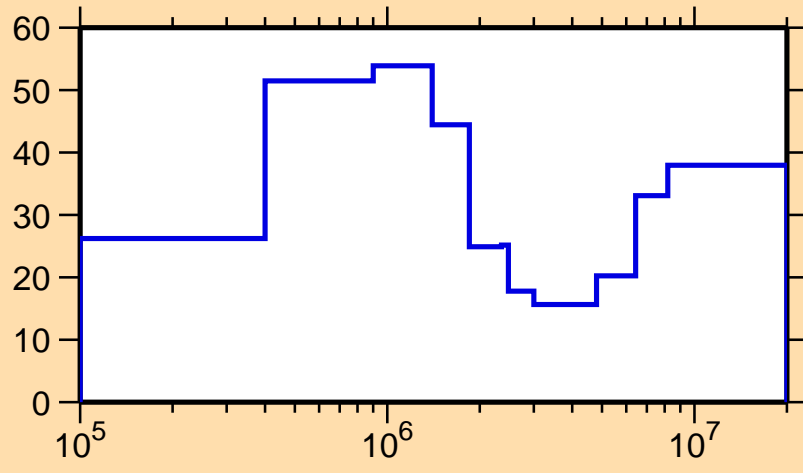
\Delta\sigma/\sigma vs. E for ^{225}\text{Po}(n,\text{tot.})
