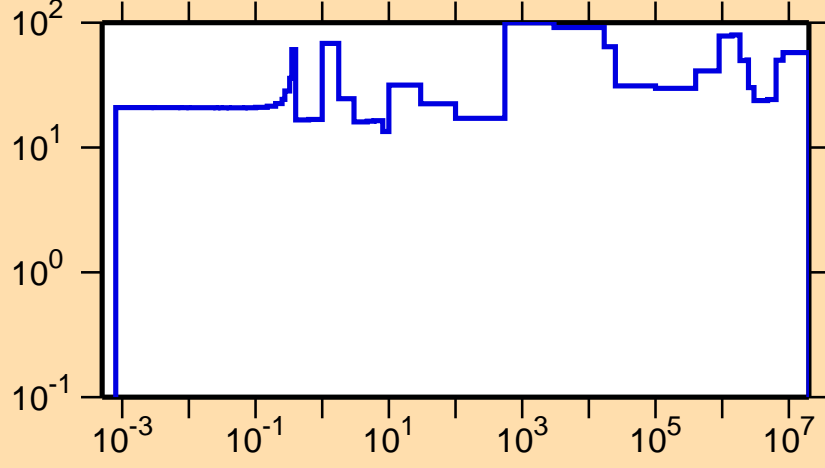
\Delta\sigma/\sigma vs. E for ^{225}\text{Po}(n,el.)
