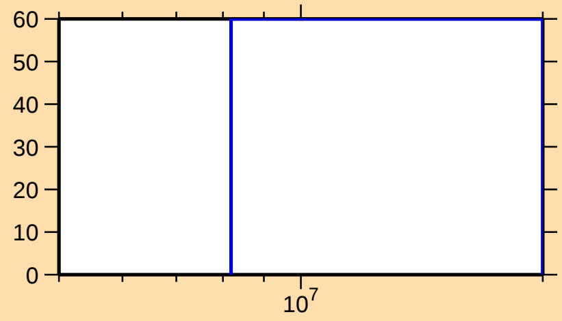
\Delta\sigma/\sigma vs. E for ^{226}\text{Po}(n,\text{ncont.})
