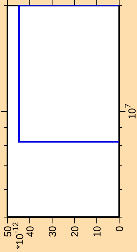
\Delta\sigma/\sigma vs. E for ^{226}\text{Po}(\text{mt } 42)
