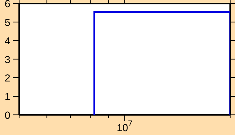
\Delta\sigma/\sigma vs. E for ^{226}\text{Po}(n,\text{el.})
