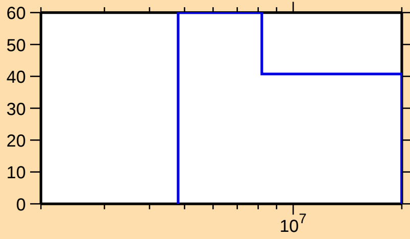
\Delta\sigma/\sigma vs. E for ^{226}\text{Po}(n,2n)
