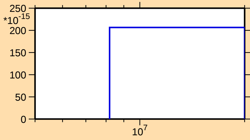
\sigma vs. E for ^{226}\text{Po}(n,2np)
