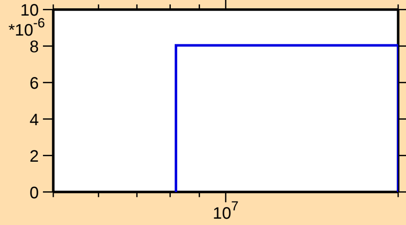
\sigma vs. E for ^{226}\text{Po}(n,p)
