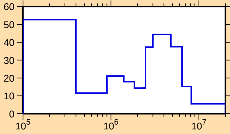
\Delta\sigma/\sigma vs. E for ^{226}\text{Po}(n,\text{el.})
