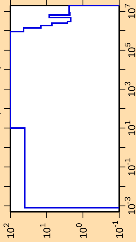
\Delta\sigma/\sigma vs. E for ^{226}\text{Po}(n,\text{nonel.})
