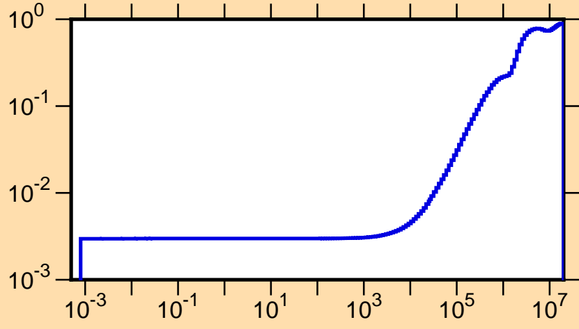
\mu vs. E for ^{227}\text{Po}(\text{mt251})
