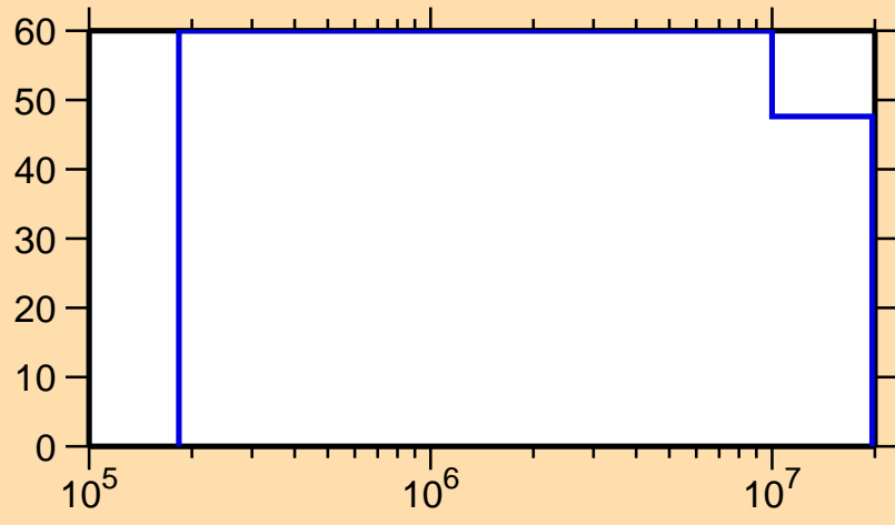
\Delta\sigma/\sigma vs. E for ^{124}\text{Pr}(n,n\text{cont.})
