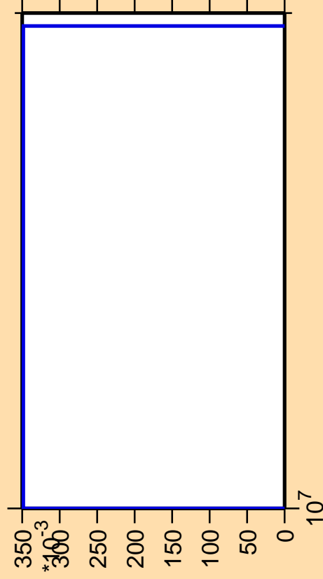
\Delta\sigma/\sigma vs. E for ^{124}\text{Pr}(n,2n\alpha)
