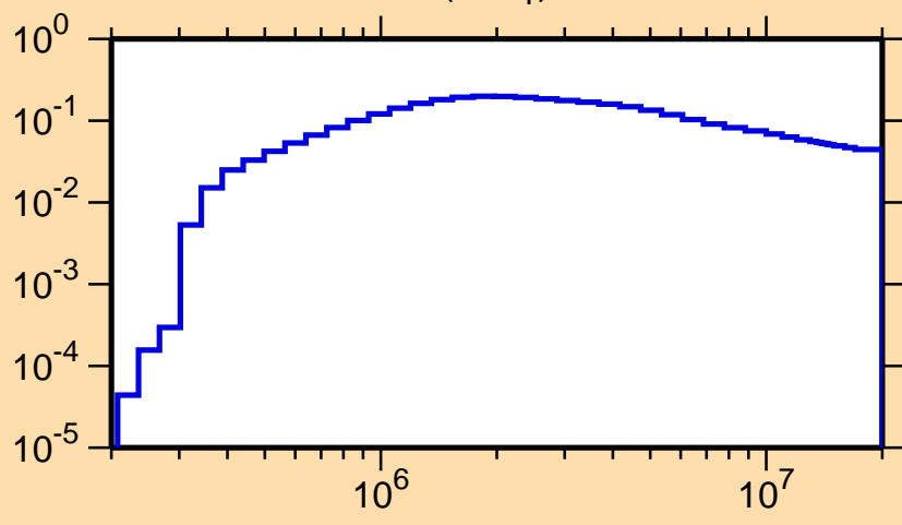
\sigma vs. E for ^{125}\text{Pr}(n,n_1)
