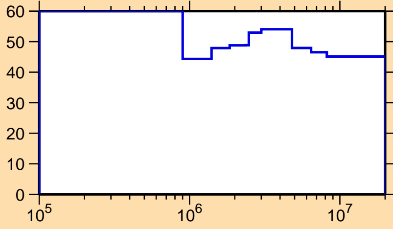
\Delta\sigma/\sigma vs. E for ^{125}\text{Pr}(n,n_1)
