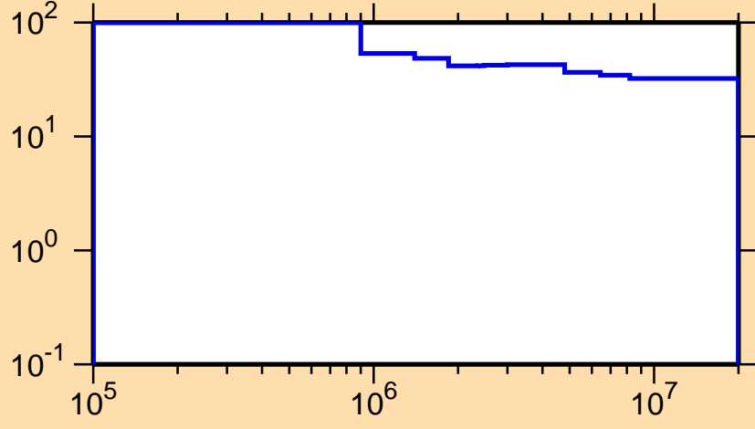
\Delta\sigma/\sigma vs. E for ^{125}\text{Pr}(n, inel.)
