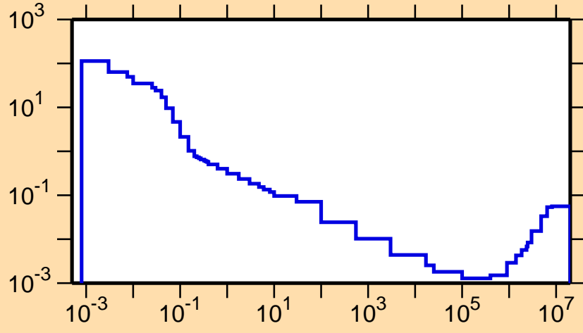
\sigma vs. E for ^{125}\text{Pr}(n,\alpha)
