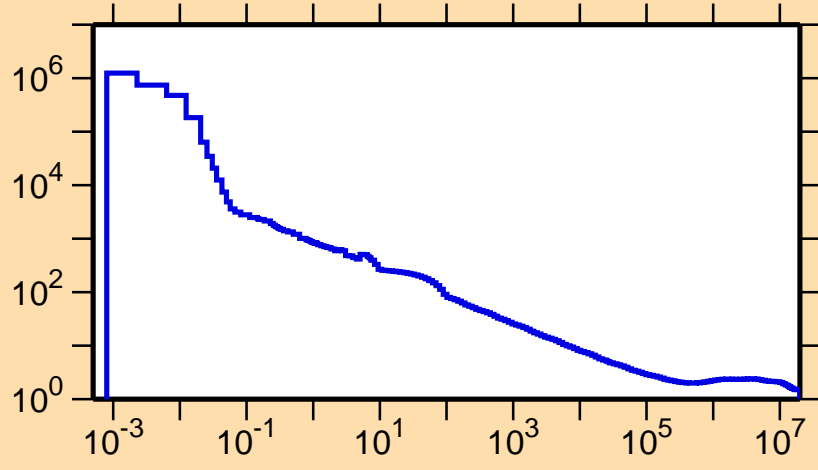
\sigma vs. E for ^{126}\text{Pr}(n,\text{nonel.})
