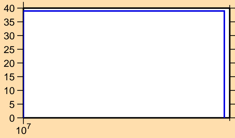
\Delta\sigma/\sigma vs. E for ^{126}\text{Pr}(n,\text{inel.})
