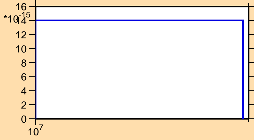
\sigma vs. E for ^{126}\text{Pr}(n,nt)
