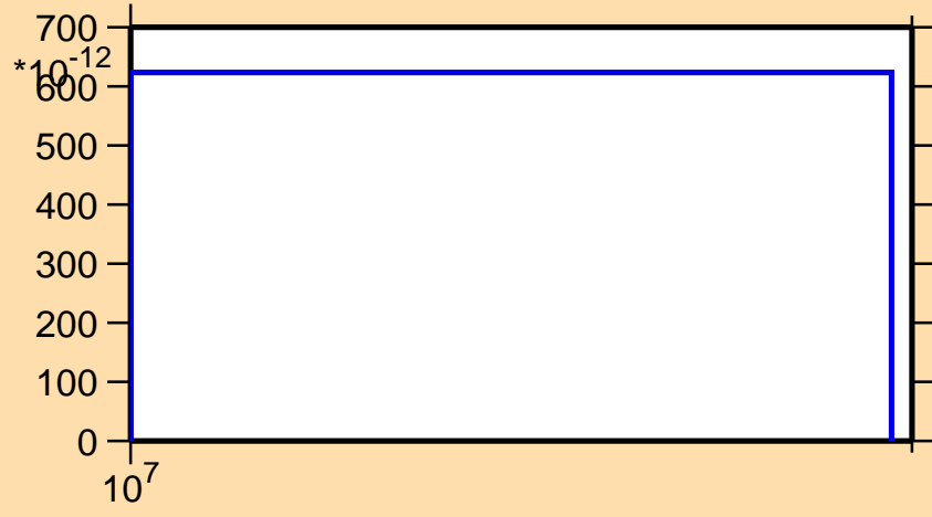
\sigma vs. E for ^{126}\text{Pr}(\text{mt } 34)
