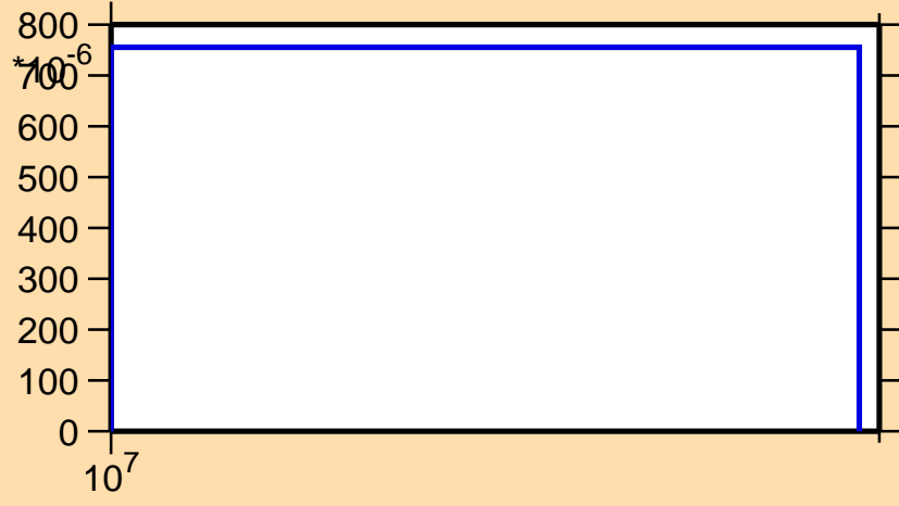
\sigma vs. E for ^{126}\text{Pr}(n,2n)
