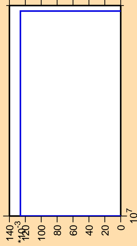
\Delta\sigma/\sigma vs. E for ^{126}\text{Pr}(n,nt)
