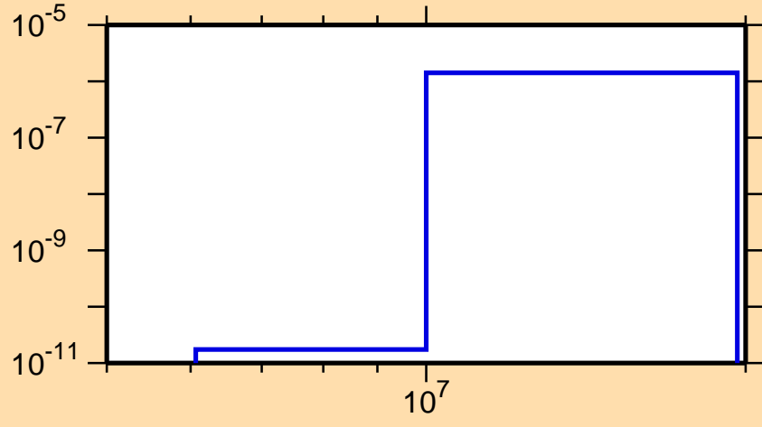
\sigma vs. E for ^{126}\text{Pr}(\text{mt117})
