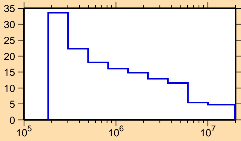
\Delta\sigma/\sigma vs. E for ^{126}\text{Pr}(n, \text{tot.})
