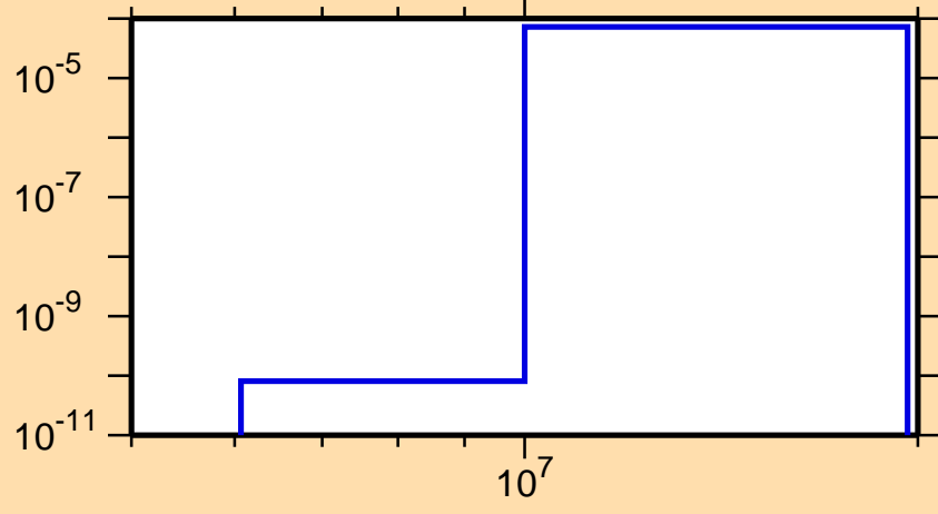
\sigma vs. E for ^{126}\text{Pr}(\text{mt } 45)
