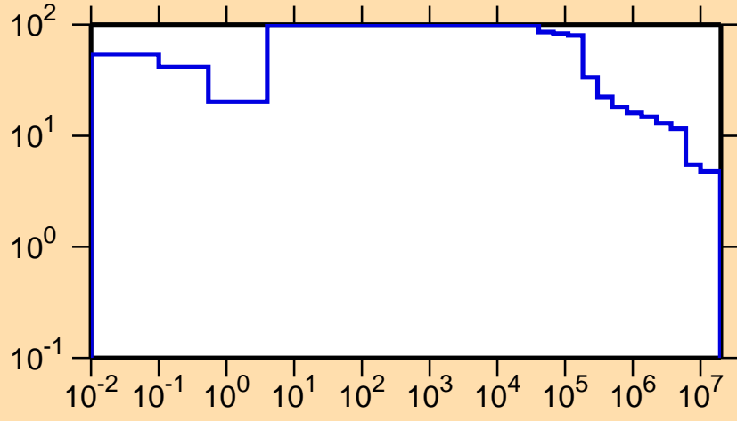
\Delta\sigma/\sigma vs. E for ^{126}\text{Pr}(n,\text{tot.})
