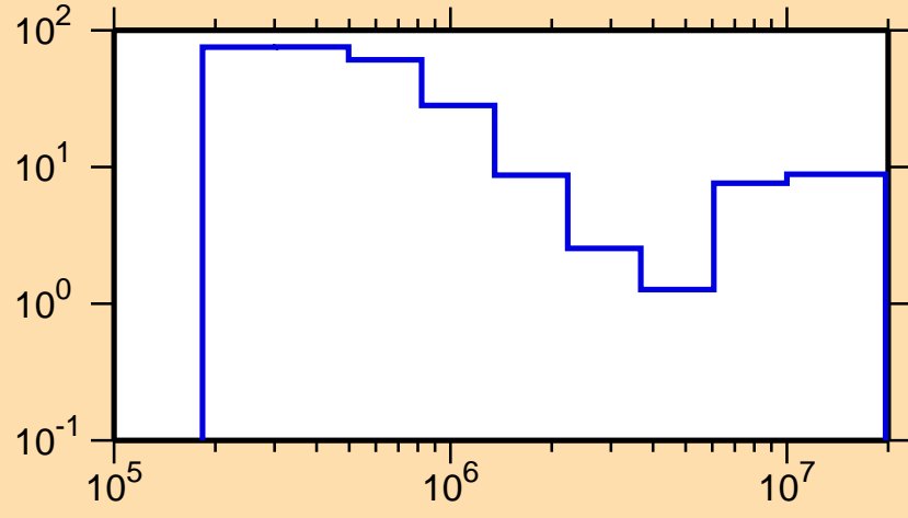
\Delta\sigma/\sigma vs. E for ^{126}\text{Pr}(n,\text{nonel.})
