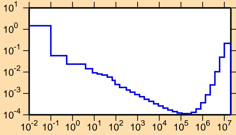
\sigma vs. E for ^{126}\text{Pr}(n,p\alpha)
