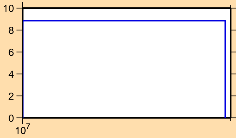
\Delta\sigma/\sigma vs. E for ^{126}\text{Pr}(n,\text{nonel.})
