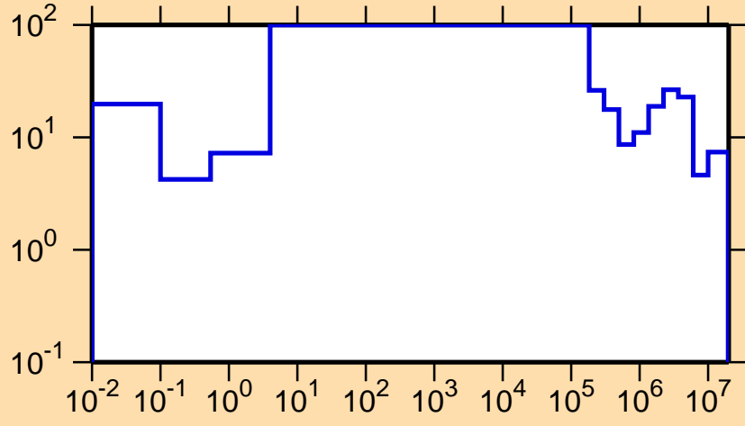
\Delta\sigma/\sigma vs. E for ^{126}\text{Pr}(n,\text{el.})
