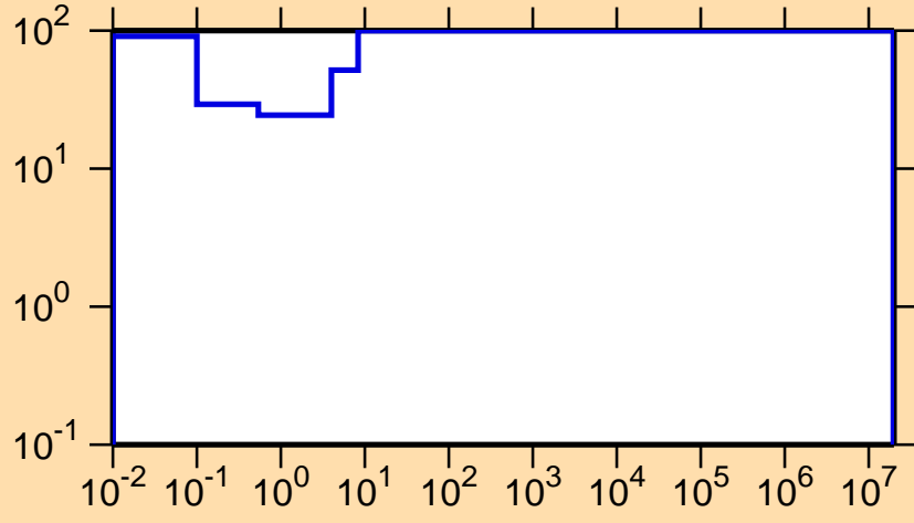
\Delta\sigma/\sigma vs. E for ^{126}\text{Pr}(n,\gamma)
