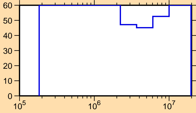
\Delta\sigma/\sigma vs. E for ^{126}\text{Pr}(n,n_1)
