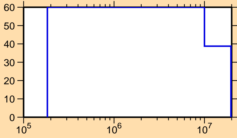
\Delta\sigma/\sigma vs. E for ^{126}\text{Pr}(n,n\text{cont.})
