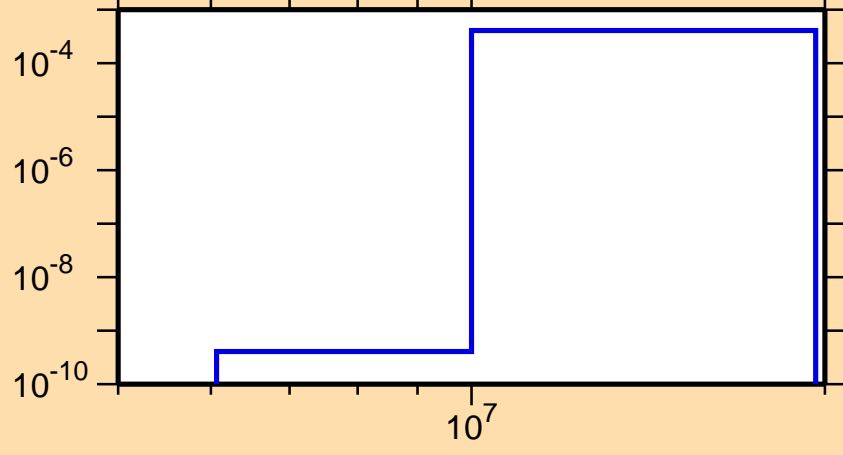
\sigma vs. E for ^{126}\text{Pr}(n,\text{pd})
