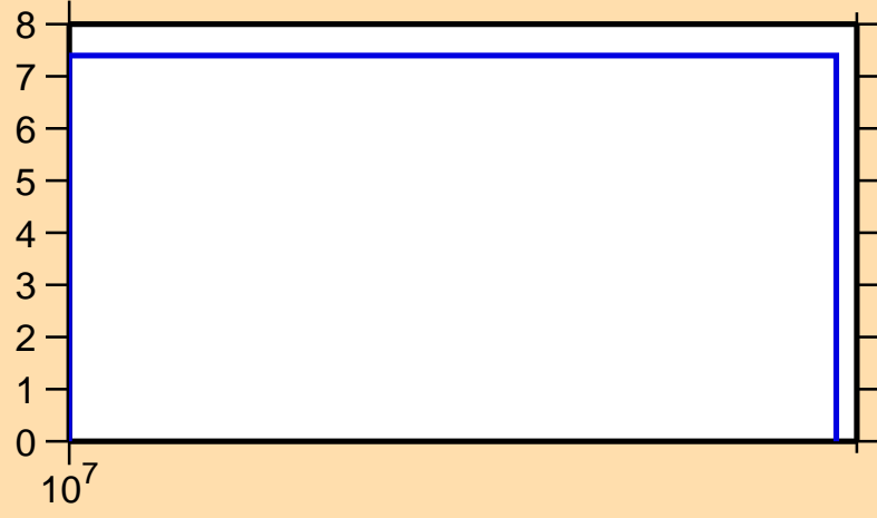
\Delta\sigma/\sigma vs. E for ^{126}\text{Pr}(n,\text{el.})
