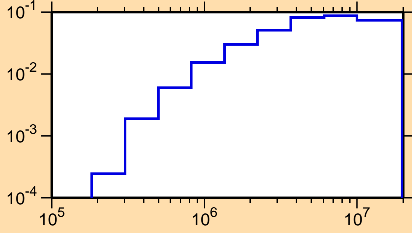
\sigma vs. E for ^{126}\text{Pr}(n,n\text{cont.})
