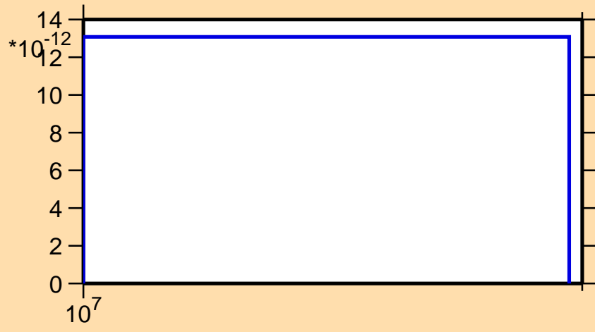
\sigma vs. E for ^{126}\text{Pr}(n,2n\alpha)
