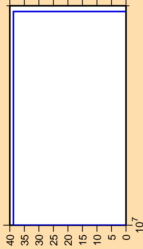
\Delta\sigma/\sigma vs. E for ^{126}\text{Pr}(n,n\text{cont.})
