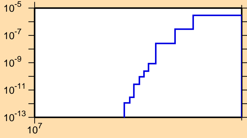
\sigma vs. E for ^{127}\text{Pr}(n,nd)
