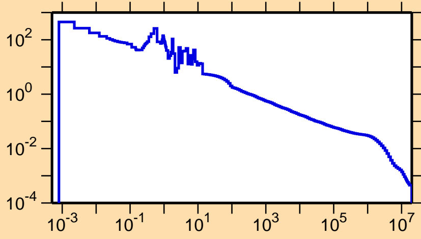
\sigma vs. E for ^{127}\text{Pr}(n,\gamma)
