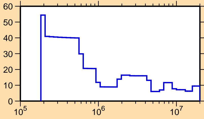
\Delta\sigma/\sigma vs. E for ^{127}\text{Pr}(n, el.)
