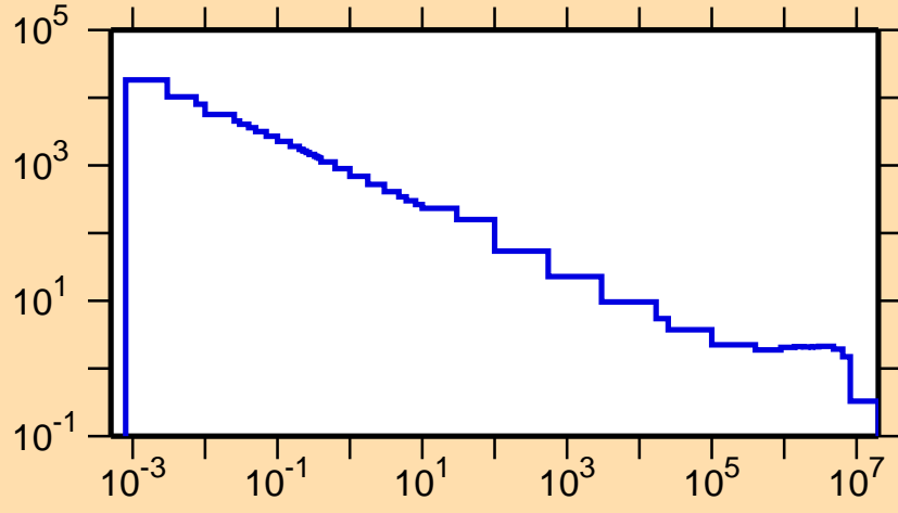
\sigma vs. E for ^{127}\text{Pr}(n,p)
