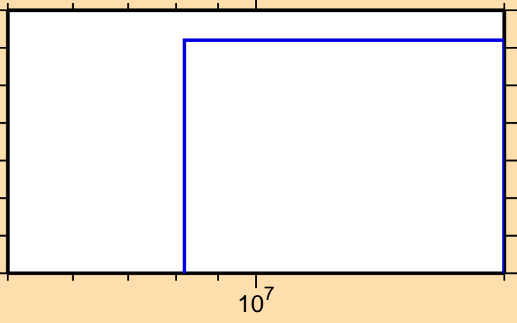
\sigma vs. E for ^{127}\text{Pr}(n,\text{pt})
