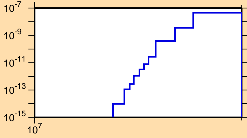
\sigma vs. E for ^{128}\text{Pr}(n,2n\alpha)
