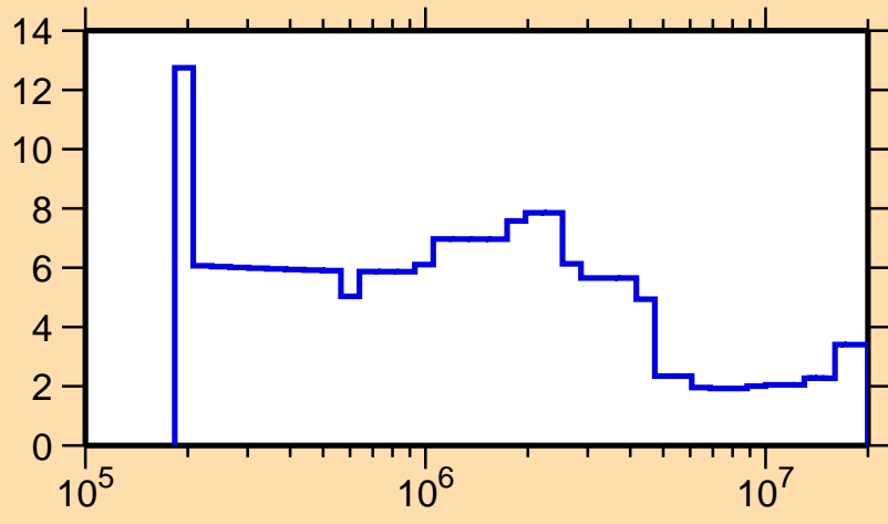
\Delta\sigma/\sigma vs. E for ^{128}\text{Pr}(n,\text{tot.})
