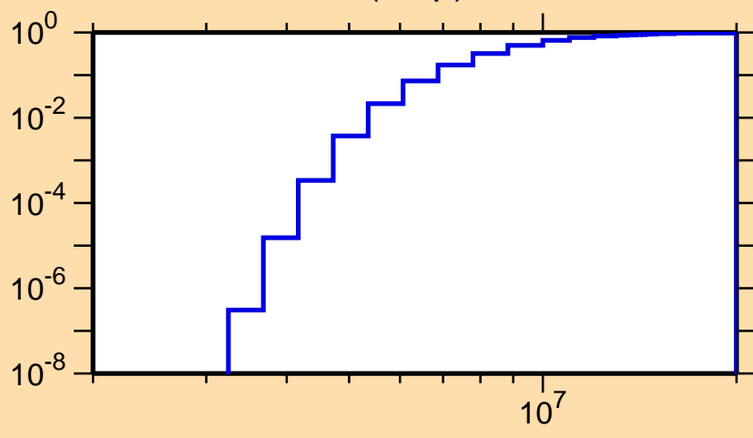
\sigma vs. E for ^{128}\text{Pr}(n,np)
