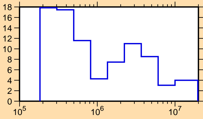
\Delta\sigma/\sigma vs. E for ^{128}\text{Pr}(n, el.)
