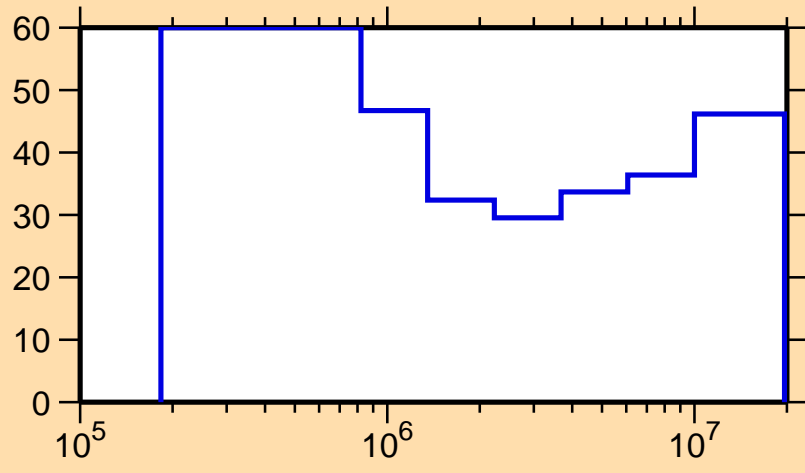
\Delta\sigma/\sigma vs. E for ^{128}\text{Pr}(n,n_1)
