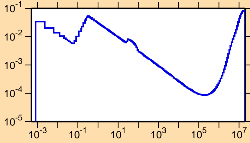
\sigma vs. E for ^{131}\text{Pr}(n,\alpha)
