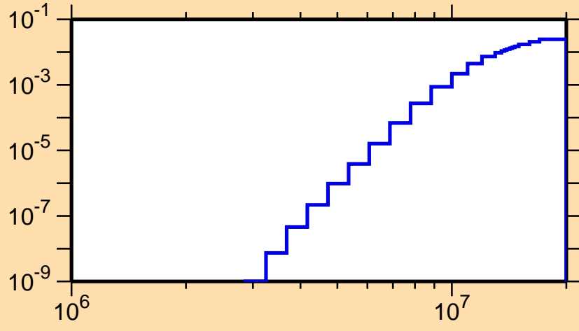
\sigma vs. E for ^{131}\text{Pr}(n,d)
