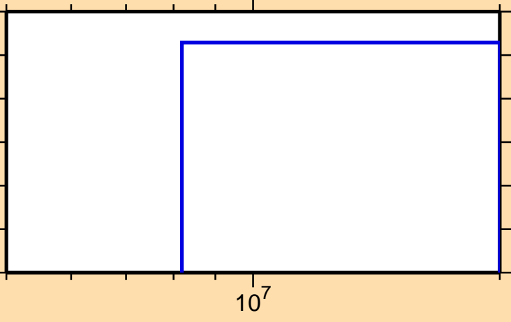
\sigma vs. E for ^{131}\text{Pr}(n,2np)
