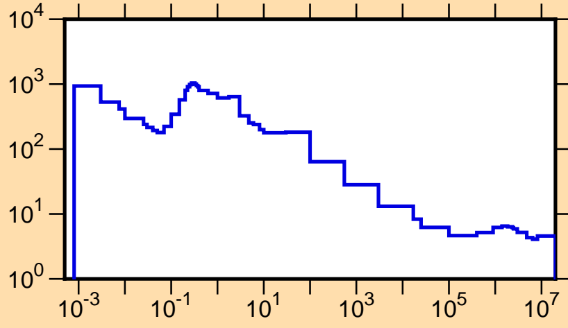
\sigma vs. E for ^{131}\text{Pr}(n,\text{tot.})
