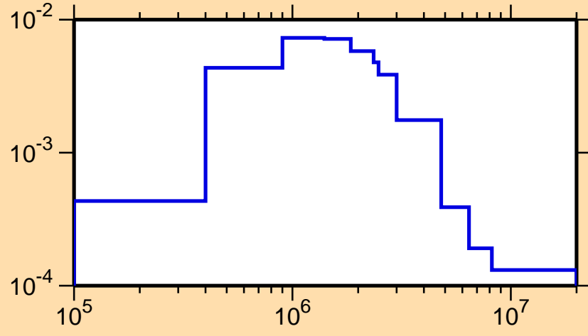
\sigma vs. E for ^{131}\text{Pr}(n,n_2)
