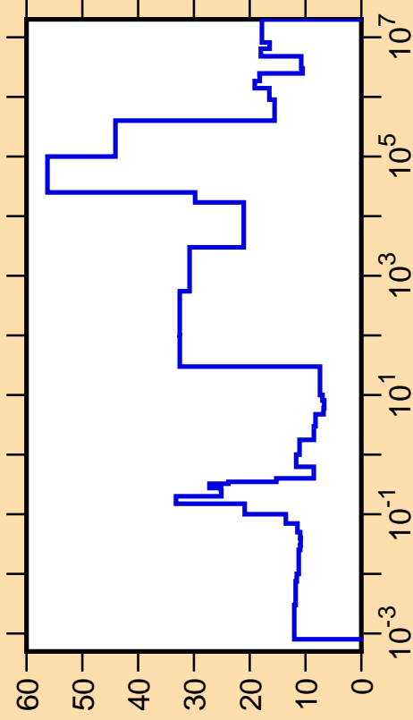
\Delta\sigma/\sigma vs. E for ^{131}\text{Pr}(n,\text{tot.})
