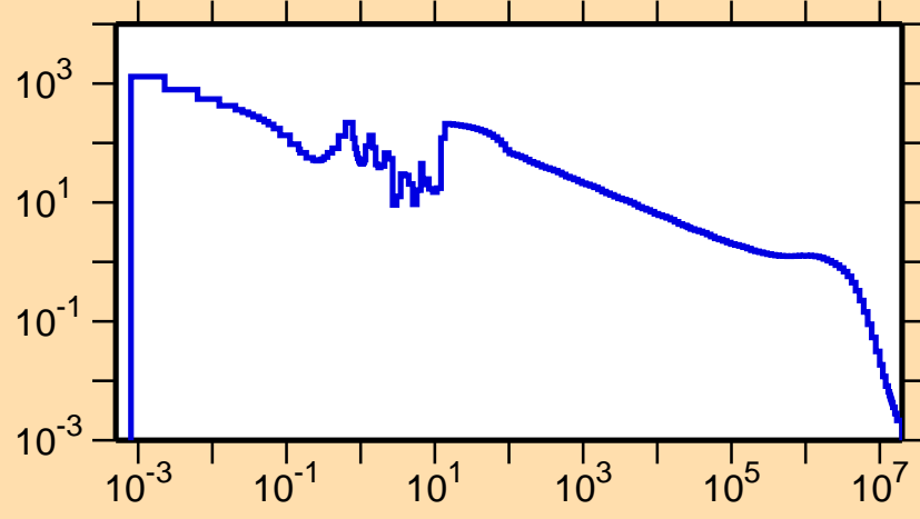
\sigma vs. E for ^{131}\text{Pr}(n,\gamma)
