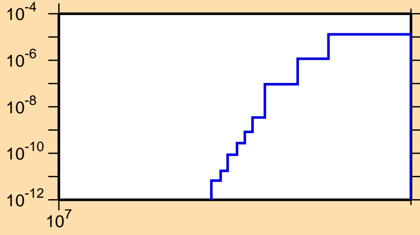
\sigma vs. E for ^{131}\text{Pr}(n,nd)
