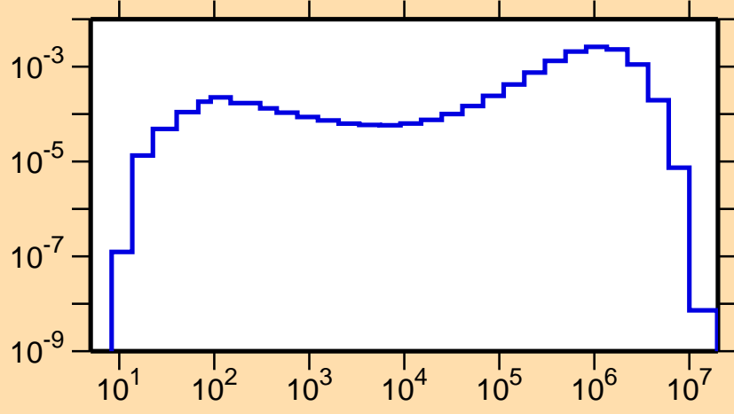
\sigma vs. E for ^{131}\text{Pr}(n,n_1)
