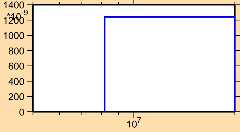
\sigma vs. E for ^{131}\text{Pr}(\text{mt } 45)
