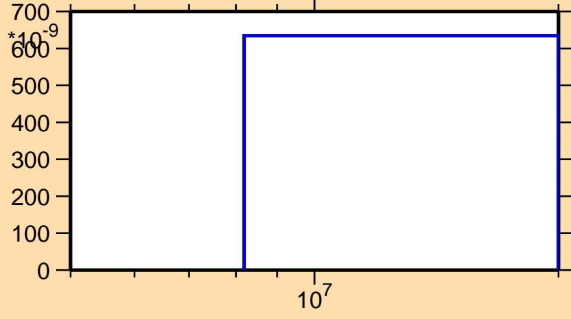
\sigma vs. E for ^{131}\text{Pr}(n,\text{pd})
