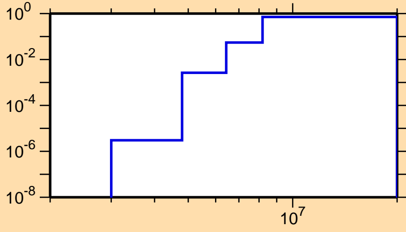
\sigma vs. E for ^{131}\text{Pr}(n,np)
