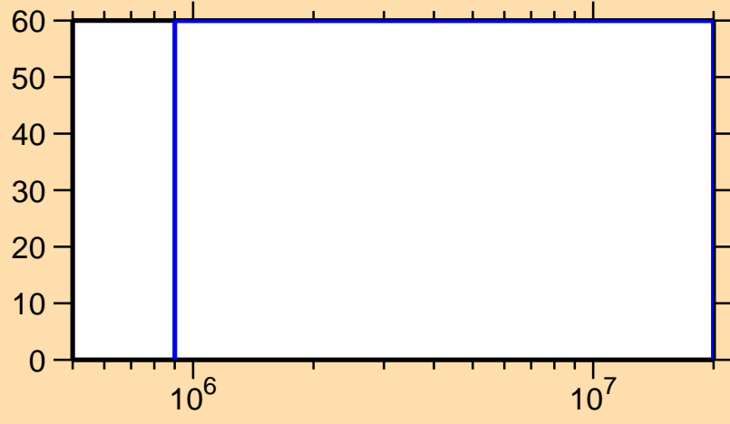
\Delta\sigma/\sigma vs. E for ^{131}\text{Pr}(n,n\text{cont.})
