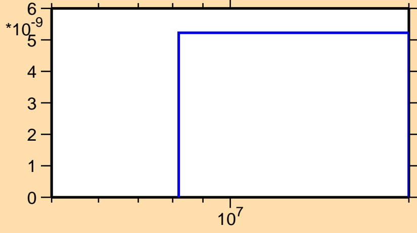
\sigma vs. E for ^{131}\text{Pr}(\text{mt117})
