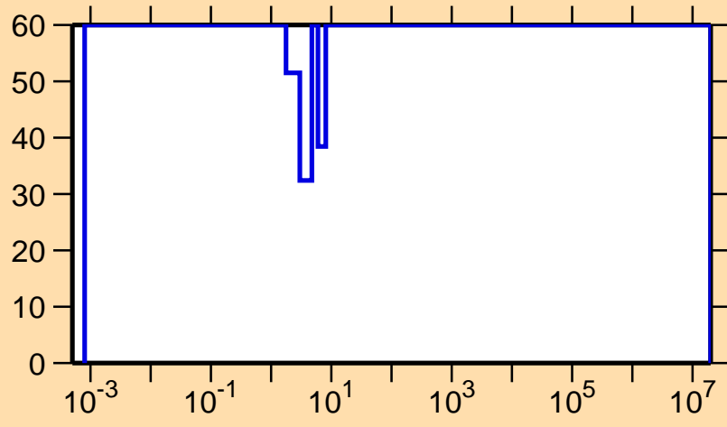
\Delta\sigma/\sigma vs. E for ^{131}\text{Pr}(n,\gamma)
