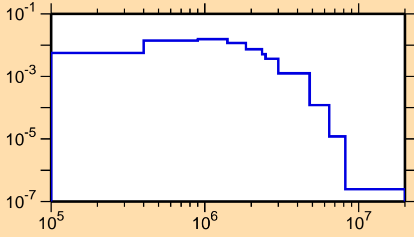
\sigma vs. E for ^{131}\text{Pr}(n,n_3)
