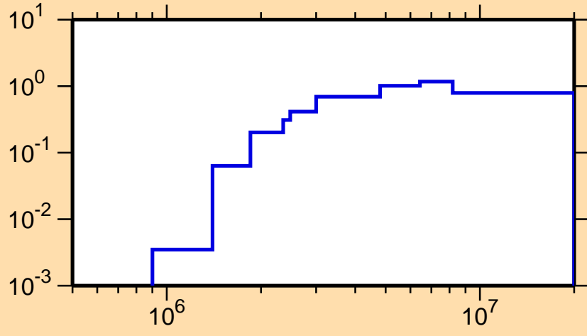
\sigma vs. E for ^{131}\text{Pr}(n,n\text{cont.})
