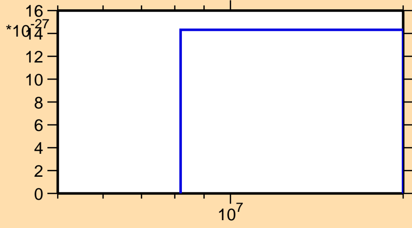
\sigma vs. E for ^{131}\text{Pr}(\text{mt } 11)
