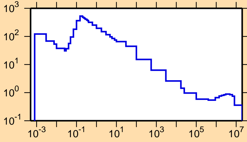
\sigma vs. E for ^{131}\text{Pr}(n,p)
