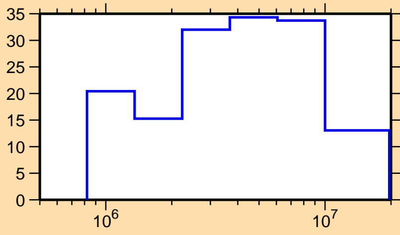
\Delta\sigma/\sigma vs. E for ^{132}\text{Pr}(n, el.)
