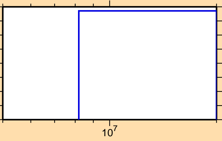
\sigma vs. E for ^{132}\text{Pr}(n,\text{nd})
