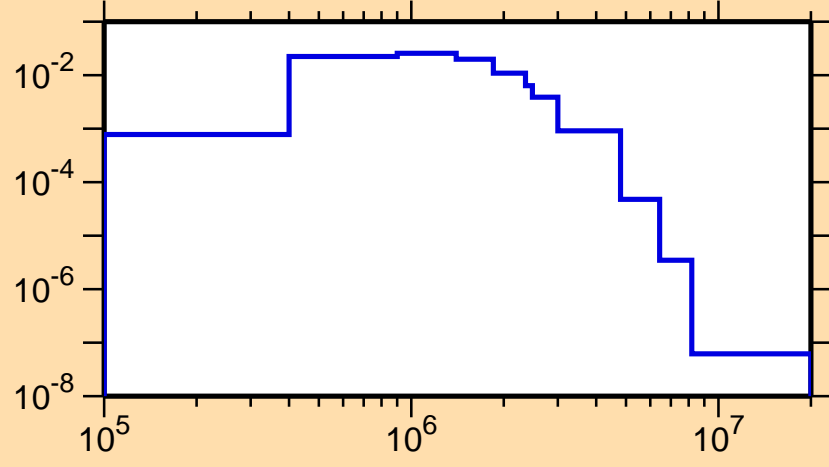
\sigma vs. E for ^{132}\text{Pr}(n,n_4)
