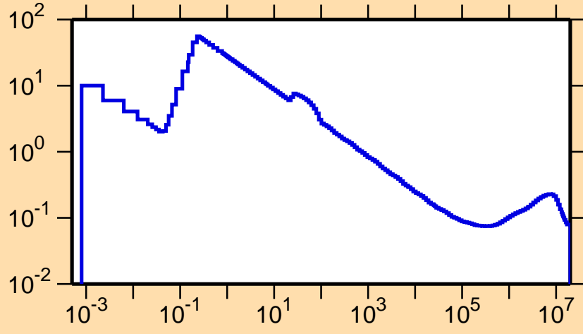
\sigma vs. E for ^{133}\text{Pr}(n,p)
