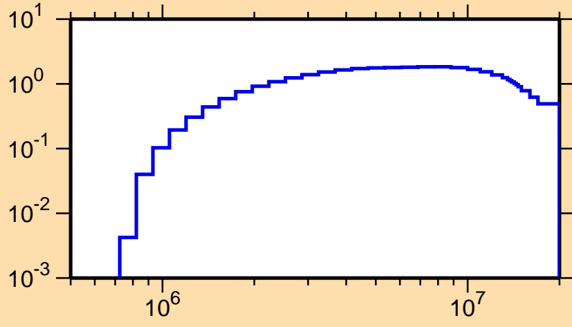
\sigma vs. E for ^{133}\text{Pr}(n,n\text{cont.})
