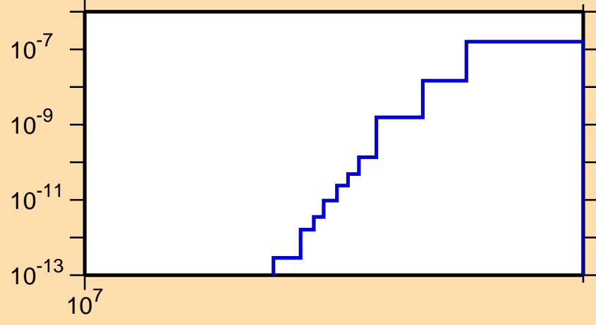
\sigma vs. E for ^{134}\text{Pr}(n,pd)
