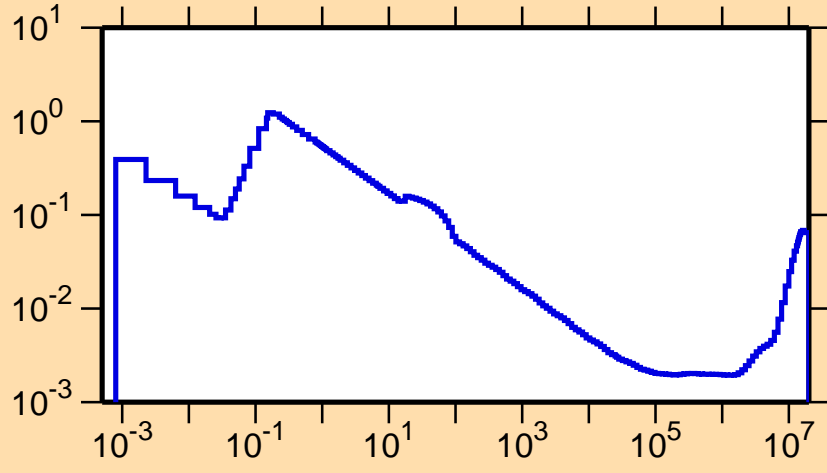
\sigma vs. E for ^{134}\text{Pr}(n,\alpha)
