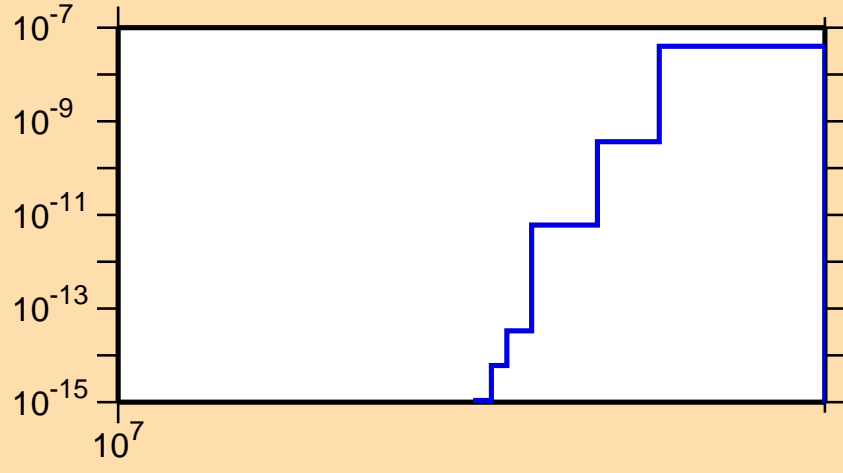
\sigma vs. E for ^{134}\text{Pr}(n,\text{pt})
