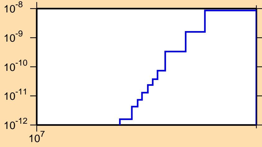
\sigma vs. E for ^{134}\text{Pr}(\text{mt117})
