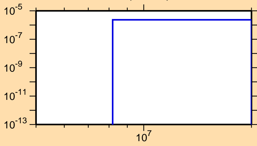
\sigma vs. E for ^{134}\text{Pr}(n,\text{He3})
