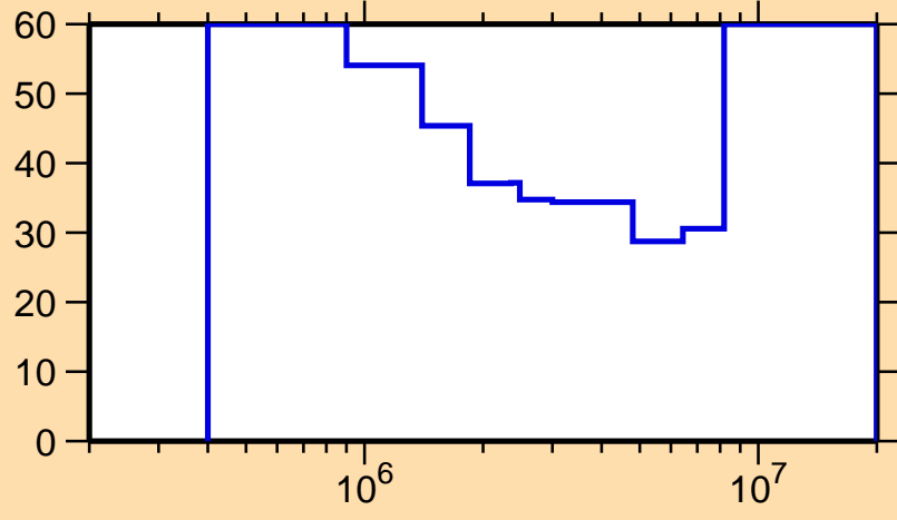
\Delta\sigma/\sigma vs. E for ^{134}\text{Pr}(n,n\text{cont.})
