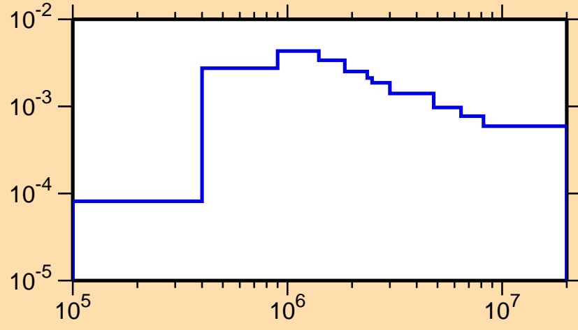
\sigma vs. E for ^{134}\text{Pr}(n,n_3)
