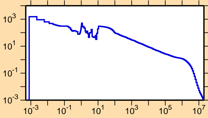
\sigma vs. E for ^{134}\text{Pr}(n,\gamma)
