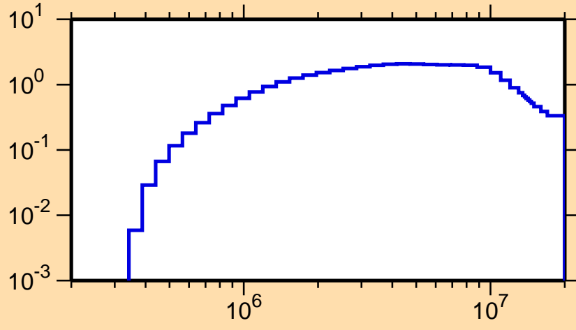
\sigma vs. E for ^{134}\text{Pr}(n,n\text{cont.})
