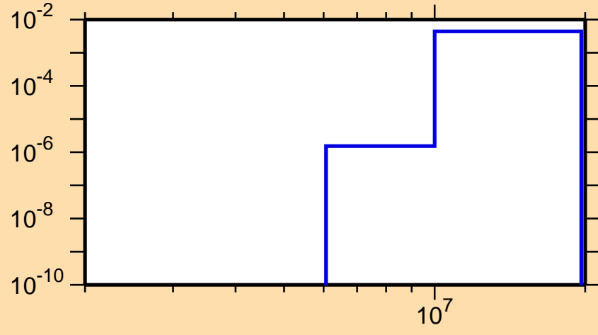
\sigma vs. E for ^{134}\text{Pr}(n,n\alpha)
