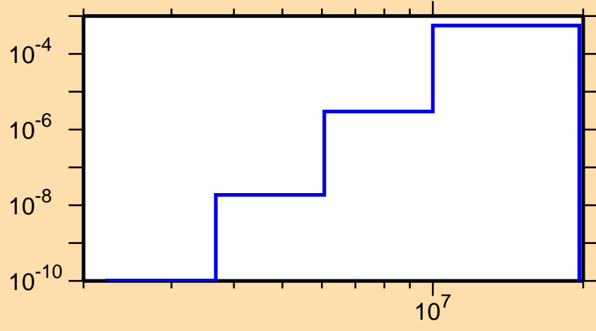
\sigma vs. E for ^{134}\text{Pr}(n,p\alpha)
