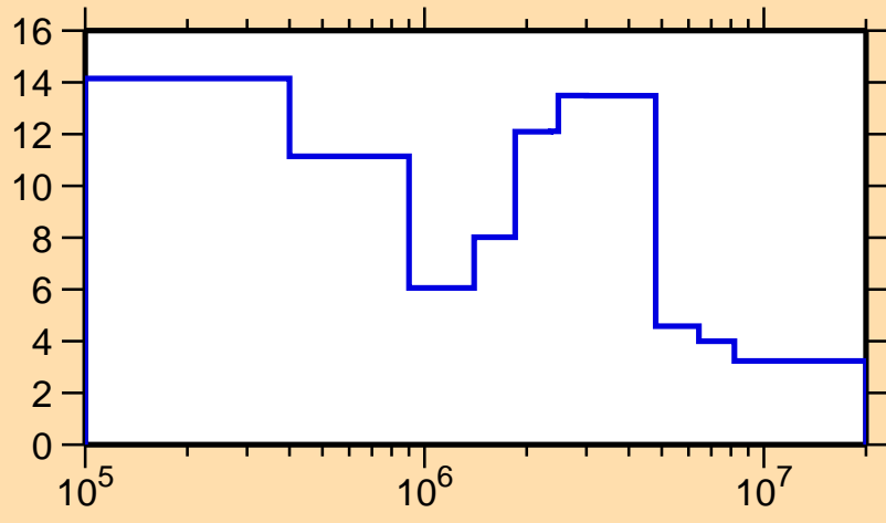
\Delta\sigma/\sigma vs. E for ^{134}\text{Pr}(n, el.)
