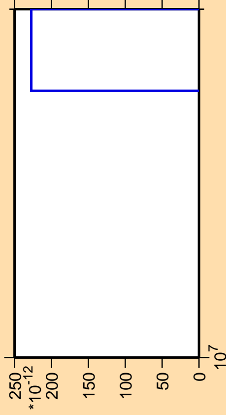
\Delta\sigma/\sigma vs. E for ^{135}\text{Pr}(\text{mt 11})
