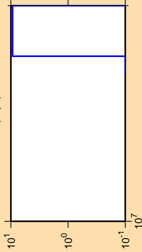
\Delta\sigma/\sigma vs. E for ^{135}\text{Pr}(n,\text{pt})
