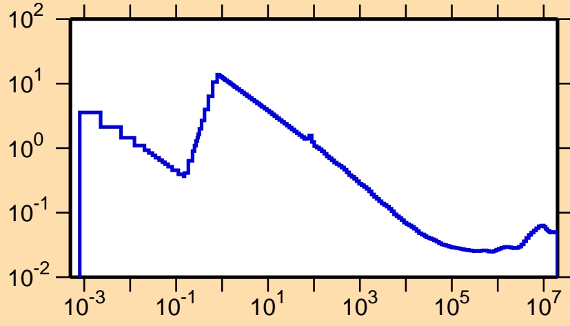
\sigma vs. E for ^{135}\text{Pr}(n,p)
