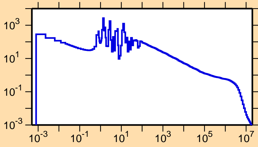
\sigma vs. E for ^{135}\text{Pr}(n,\gamma)
