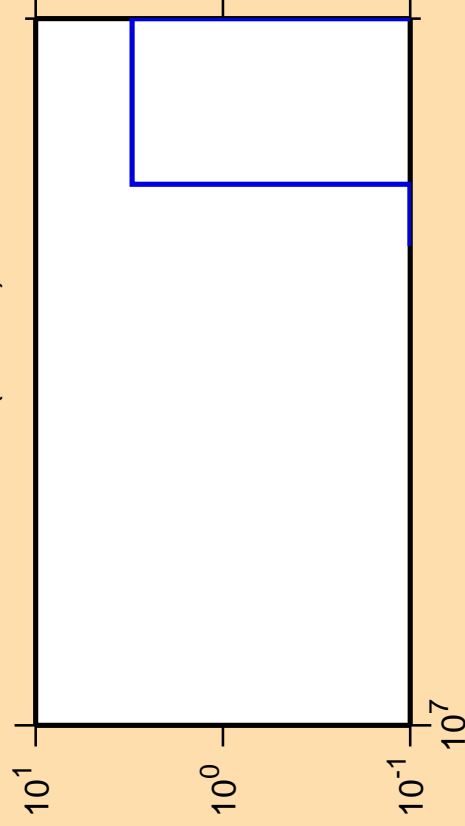
\Delta\sigma/\sigma vs. E for ^{135}\text{Pr}(\text{mt } 34)
