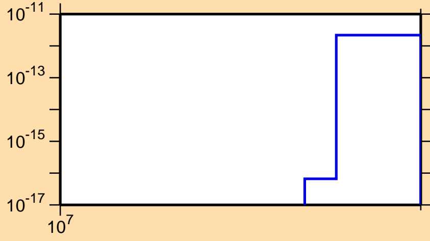
\sigma vs. E for ^{135}\text{Pr}(n,\text{pt})
