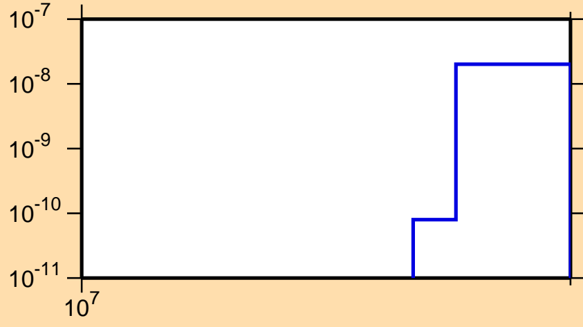
\sigma vs. E for ^{135}\text{Pr}(n,2n\alpha)
