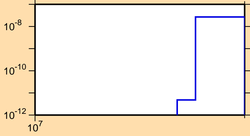
\sigma vs. E for ^{135}\text{Pr}(n,nt)
