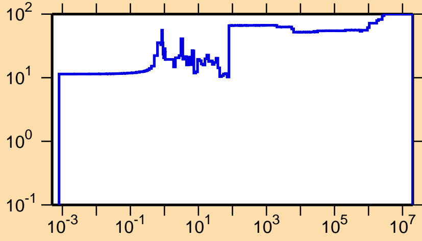
\Delta\sigma/\sigma vs. E for ^{135}\text{Pr}(n,\gamma)
