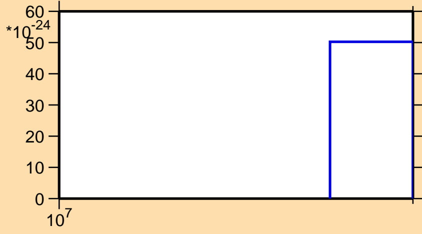
\sigma vs. E for ^{135}\text{Pr}(\text{mt 11})
