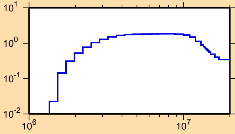
\sigma vs. E for ^{135}\text{Pr}(n,n\text{cont.})
