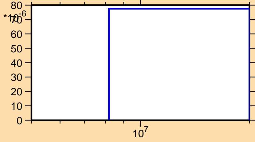
\sigma vs. E for ^{135}\text{Pr}(n,t)
