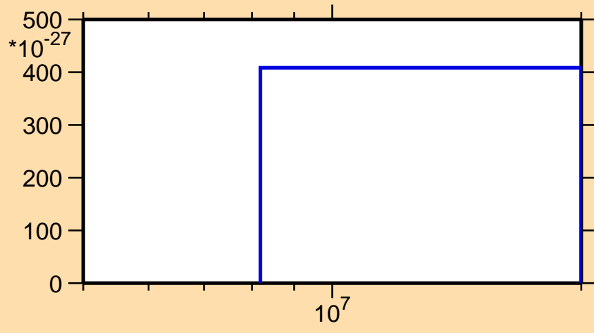
\sigma vs. E for ^{135}\text{Pr}(\text{mt } 11)
