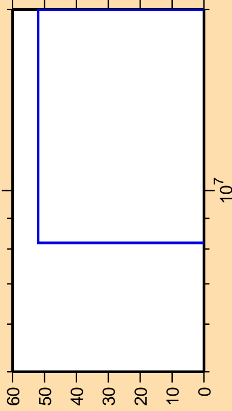
\Delta\sigma/\sigma vs. E for ^{136}\text{Pr}(\text{mt } 45)
