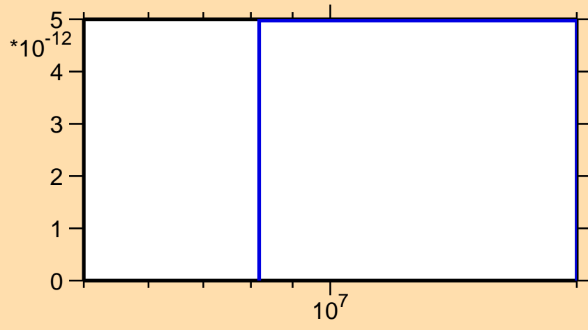
\sigma vs. E for ^{136}\text{Pr}(\text{mt117})
