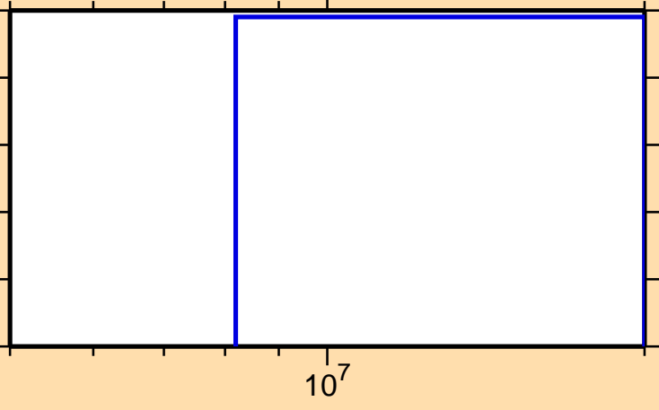
\sigma vs. E for ^{136}\text{Pr}(n,pd)
