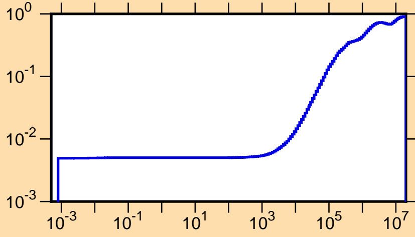
\mu vs. E for ^{137}\text{Pr}(\text{mt251})
