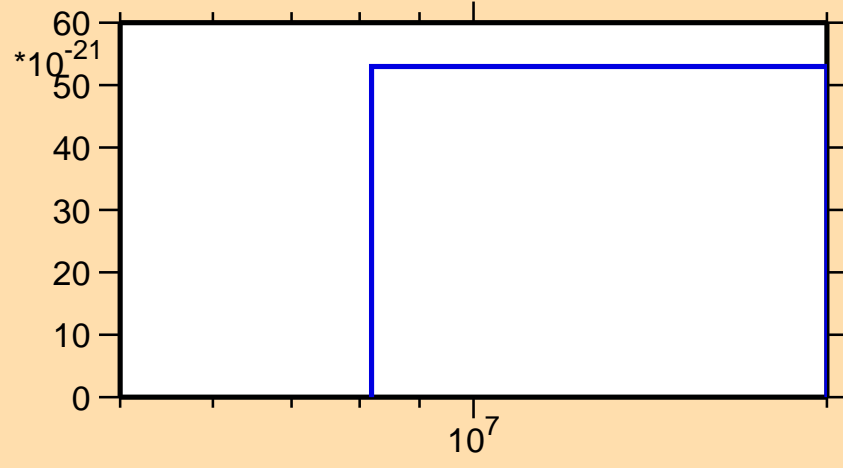
\sigma vs. E for ^{137}\text{Pr}(\text{mt } 11)
