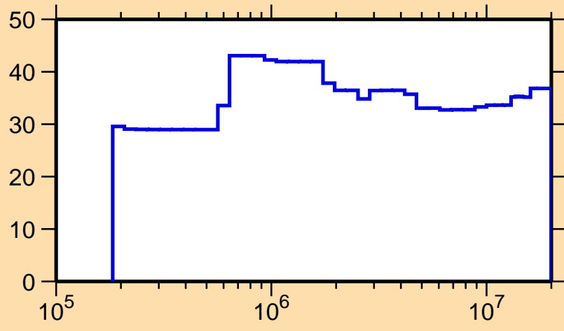
\Delta\sigma/\sigma vs. E for ^{138}\text{Pr}(n,n_1)
