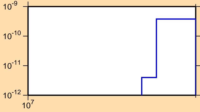
\sigma vs. E for ^{138}\text{Pr}(n,\text{pd})
