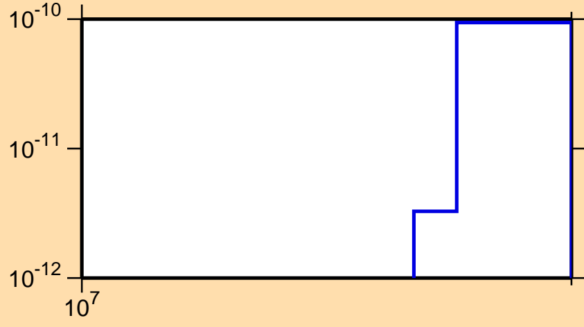
\sigma vs. E for ^{138}\text{Pr}(\text{mt } 45)
