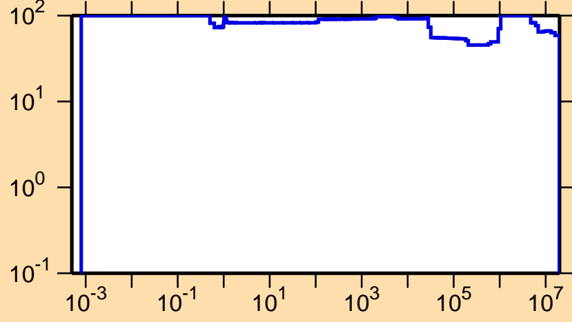
\Delta\sigma/\sigma vs. E for ^{138}\text{Pr}(n,p)
