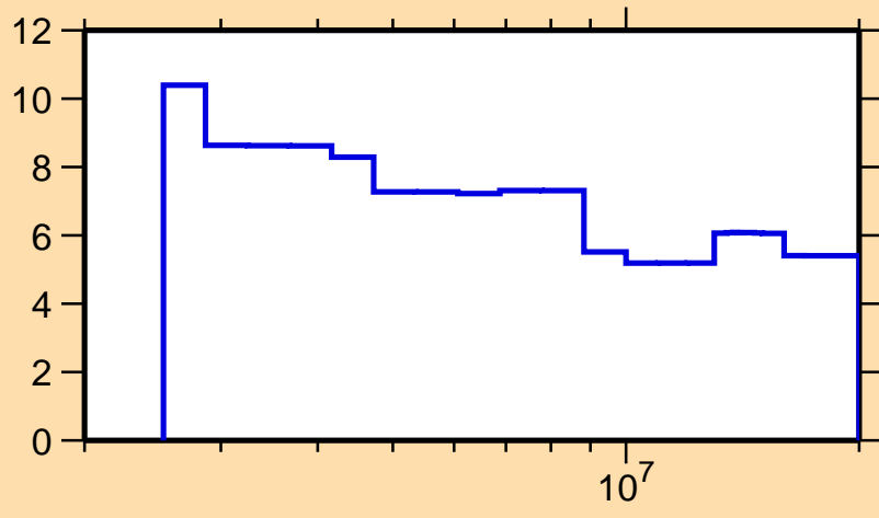
\Delta\sigma/\sigma vs. E for ^{138}\text{Pr}(n,n\text{onl.})
