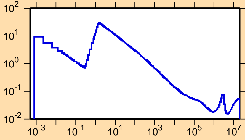
\sigma vs. E for ^{138}\text{Pr}(n,p)
