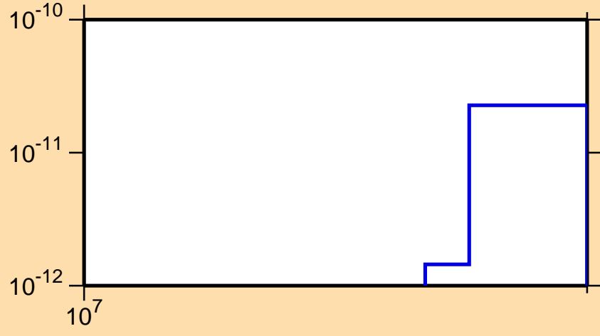
\sigma vs. E for ^{138}\text{Pr}(\text{mt117})
