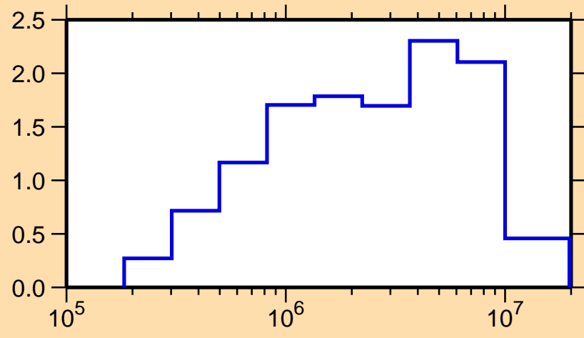
\sigma vs. E for ^{138}\text{Pr}(n,\text{inel.})
