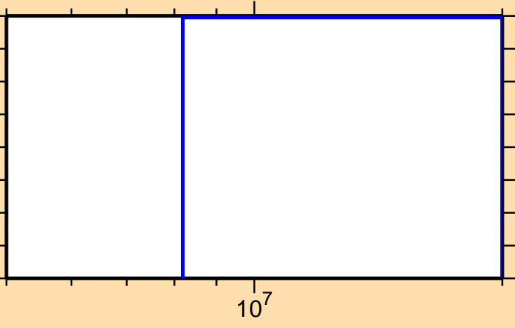
\sigma vs. E for ^{138}\text{Pr}(n,3n)
