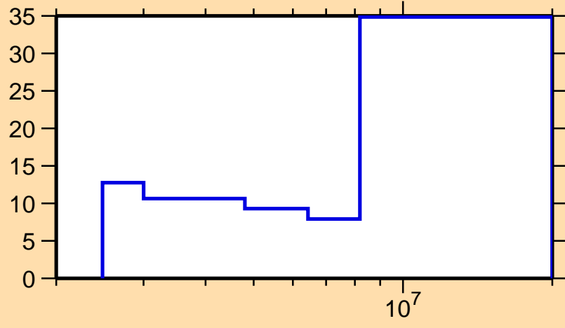
\Delta\sigma/\sigma vs. E for ^{138}\text{Pr}(n,n\text{cont.})
