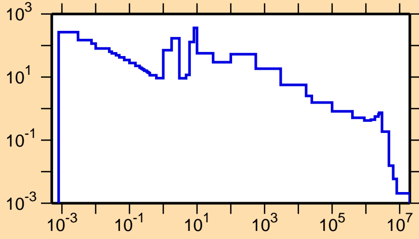
\sigma vs. E for ^{138}\text{Pr}(n,\gamma)
