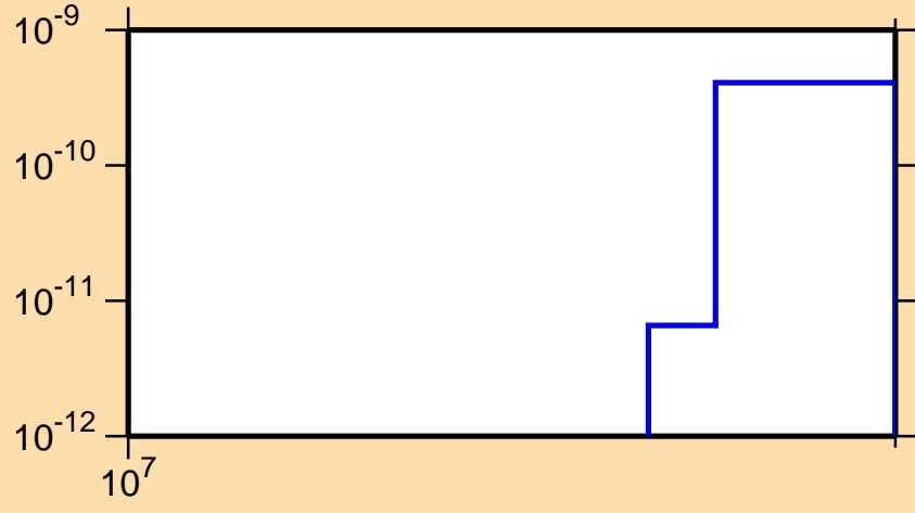
\sigma vs. E for ^{138}\text{Pr}(n,pd)
