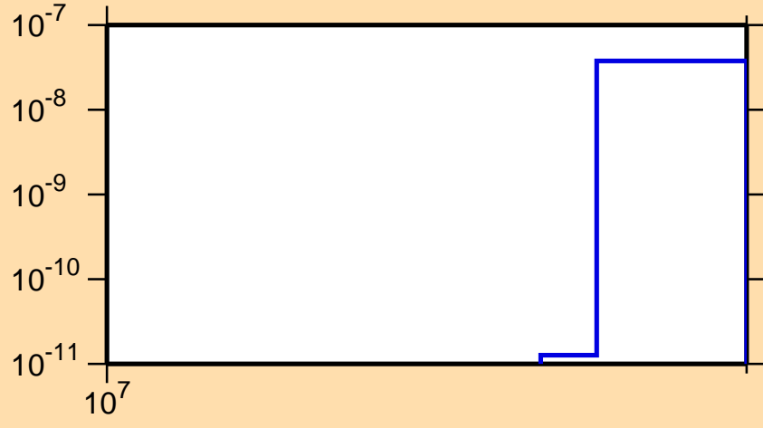
\sigma vs. E for ^{138}\text{Pr}(n,nt)
