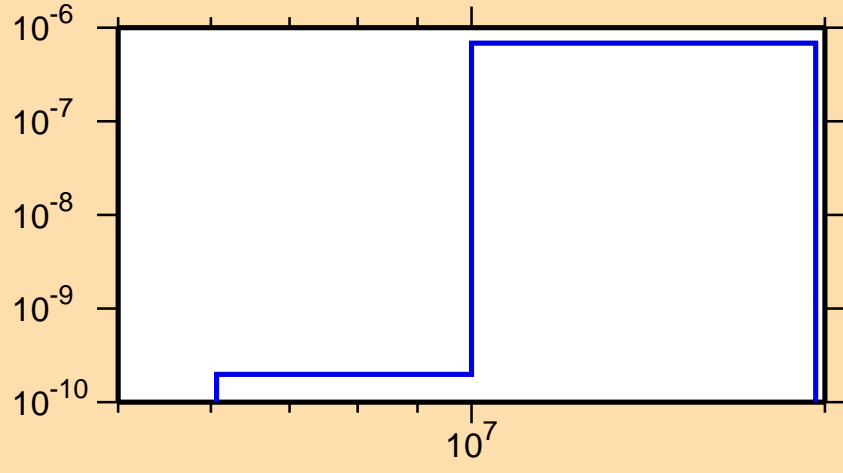
\sigma vs. E for ^{138}\text{Pr}(n,p\alpha)
