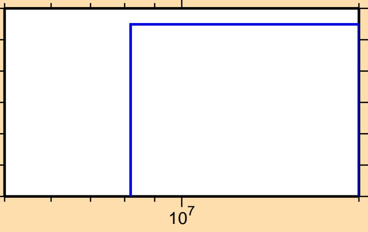
\sigma vs. E for ^{138}\text{Pr}(n,3n)
