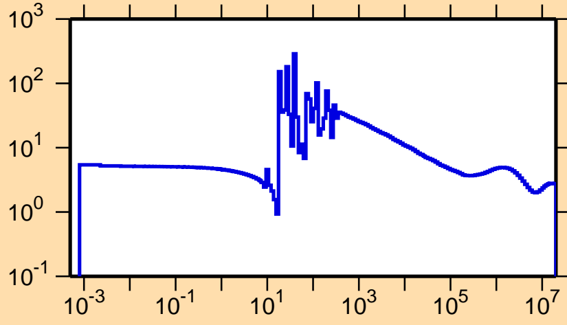
\sigma vs. E for ^{139}\text{Pr}(n,\text{el.})
