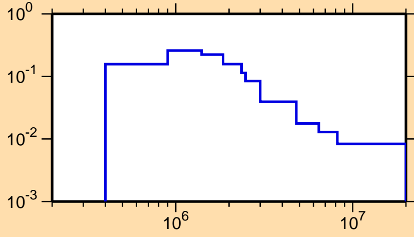
\sigma vs. E for ^{139}\text{Pr}(n,n_2)
