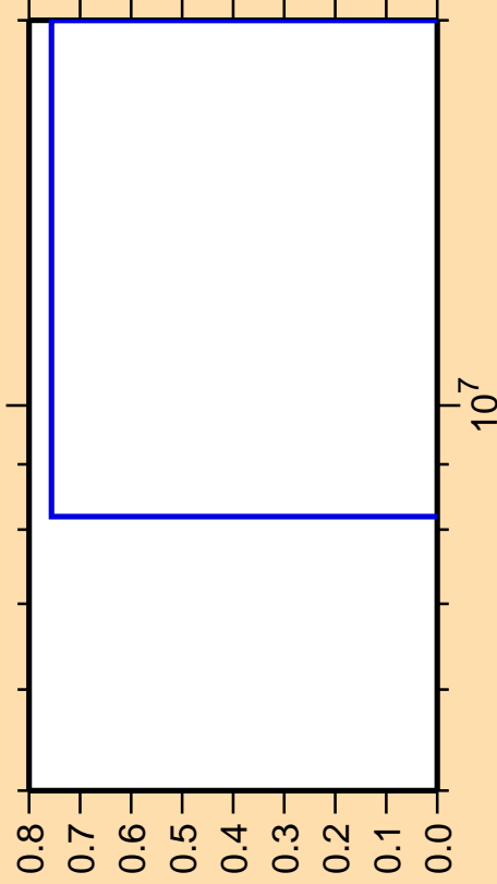
\Delta\sigma/\sigma vs. E for ^{139}\text{Pr}(n,pd)
