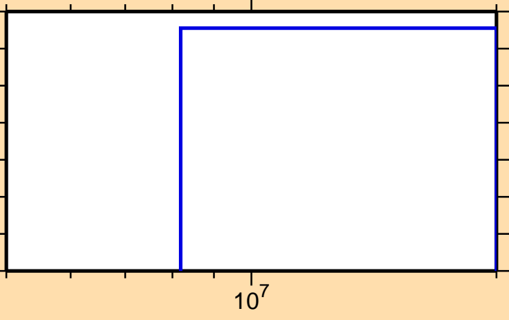
\sigma vs. E for ^{139}\text{Pr}(n,\text{nd})
