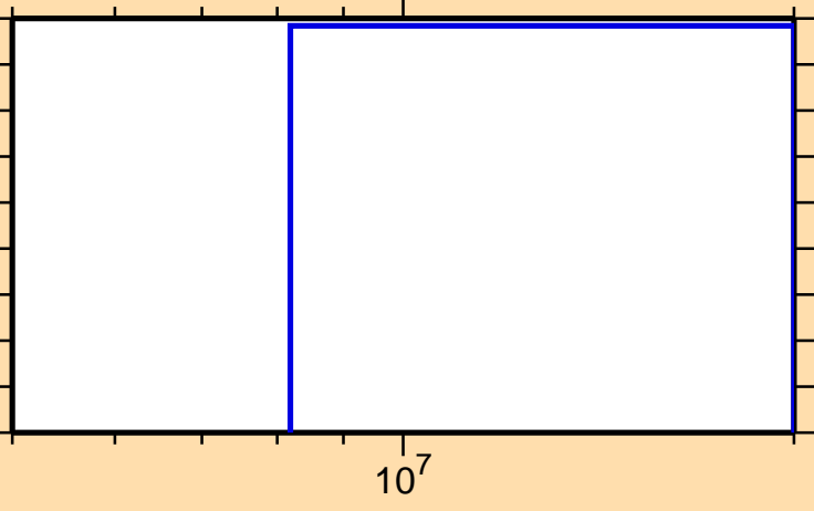
\sigma vs. E for ^{139}\text{Pr}(n,3n)
