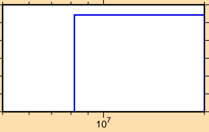
\sigma vs. E for ^{139}\text{Pr}(n,2np)
