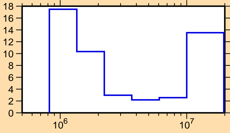
\Delta\sigma/\sigma vs. E for ^{140}\text{Pr}(n,n\text{cont.})
