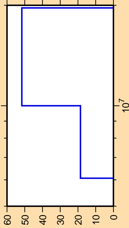
\Delta\sigma/\sigma vs. E for ^{141}\text{Pr}(n,t)
