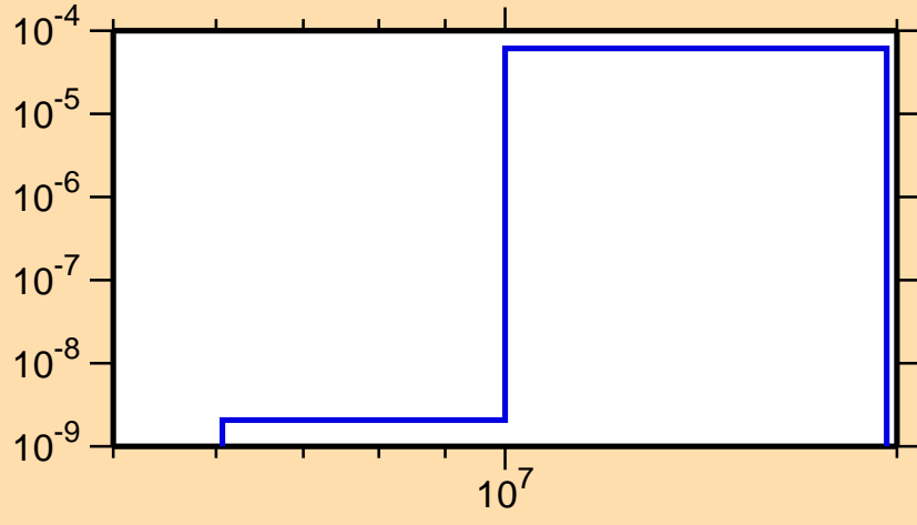
\sigma vs. E for ^{141}\text{Pr}(n,n\alpha)
