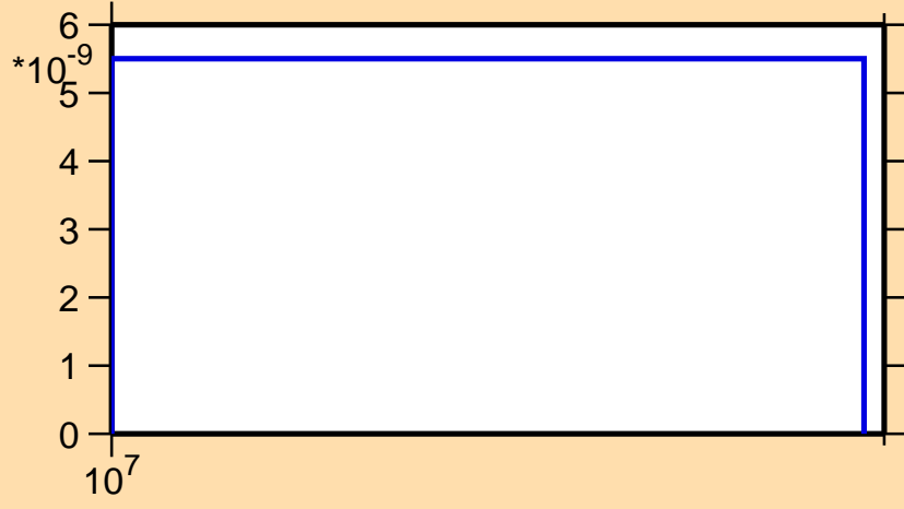
\sigma vs. E for ^{141}\text{Pr}(n,2np)
