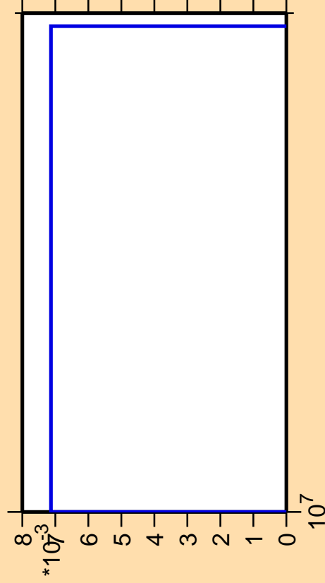
\Delta\sigma/\sigma vs. E for ^{141}\text{Pr}(n,pd)
