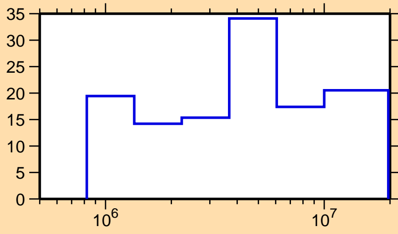
\Delta\sigma/\sigma vs. E for ^{141}\text{Pr}(n,n_1)
