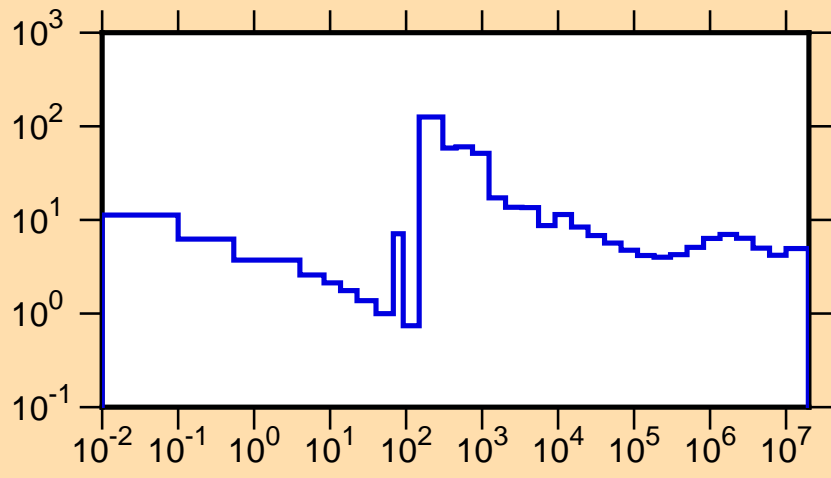
\sigma vs. E for ^{141}\text{Pr}(n,\text{tot.})
