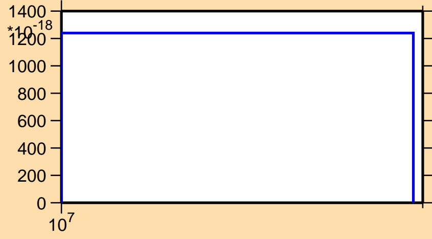
\sigma vs. E for ^{141}\text{Pr}(n,pd)
