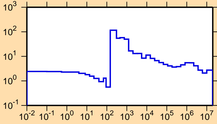
\sigma vs. E for ^{141}\text{Pr}(n,\text{el.})
