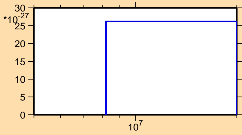
\sigma vs. E for ^{141}\text{Pr}(\text{mt } 11)
