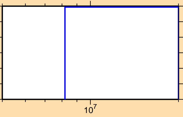
\sigma vs. E for ^{141}\text{Pr}(n,\text{He3})
