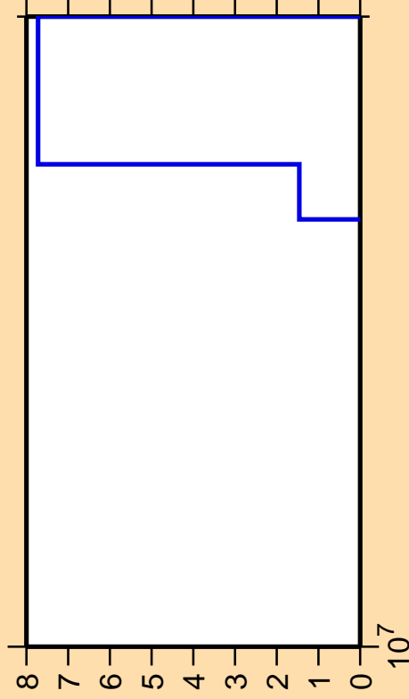
\Delta\sigma/\sigma vs. E for ^{144}\text{Pr}(\text{mt117})
