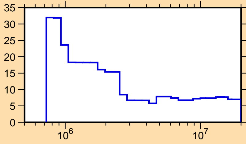
\Delta\sigma/\sigma vs. E for ^{144}\text{Pr}(n,n\text{onel.})
