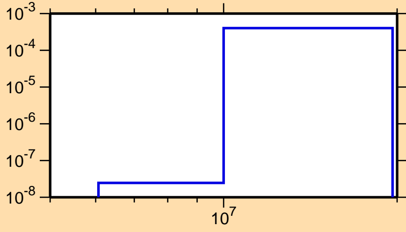
\sigma vs. E for ^{144}\text{Pr}(n,t)
