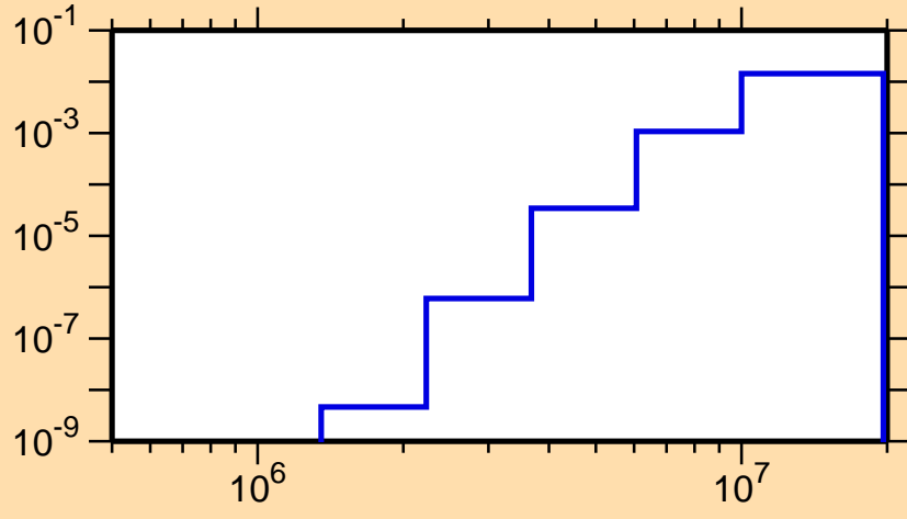
\sigma vs. E for ^{144}\text{Pr}(n,p)
