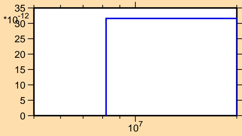
\sigma vs. E for ^{144}\text{Pr}(n,p\alpha)
