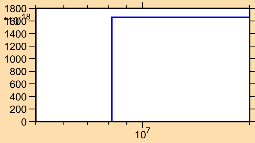
\sigma vs. E for ^{144}\text{Pr}(n,3n\alpha)
