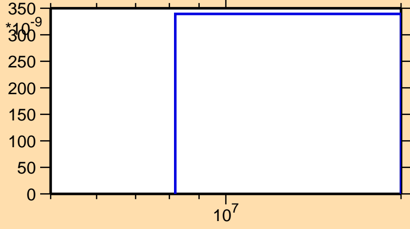
\sigma vs. E for ^{144}\text{Pr}(n,2np)
