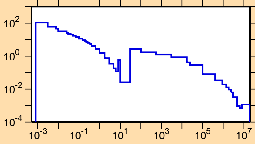
\sigma vs. E for ^{144}\text{Pr}(n,\gamma)
