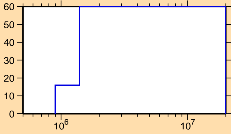
\Delta\sigma/\sigma vs. E for ^{144}\text{Pr}(n,p)
