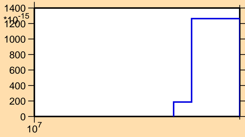
\sigma vs. E for ^{144}\text{Pr}(\text{mt117})
