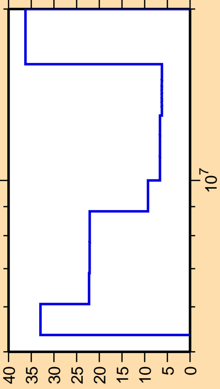
\Delta\sigma/\sigma vs. E for ^{144}\text{Pr}(n,2n)
