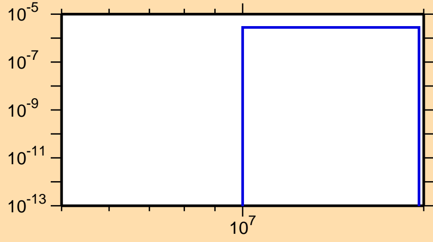
\sigma vs. E for ^{144}\text{Pr}(n,\text{nd})
