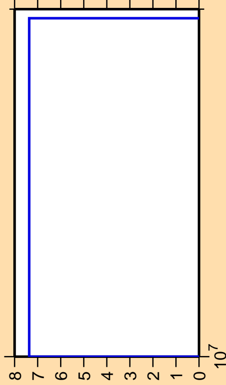
\Delta\sigma/\sigma vs. E for ^{144}\text{Pr}(n,3n)
