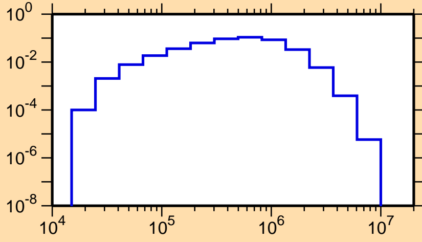
\sigma vs. E for ^{144}\text{Pr}(n,n_2)
