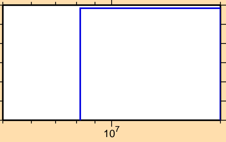
\sigma vs. E for ^{144}\text{Pr}(\text{mt } 42)
